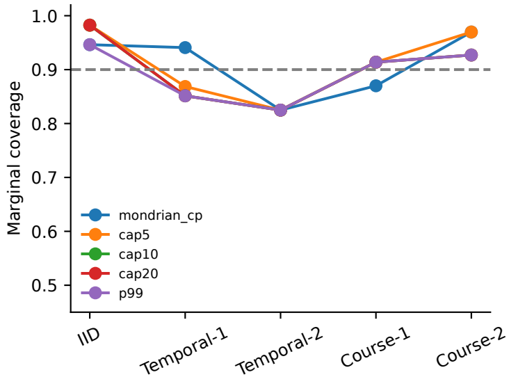
Logistic
