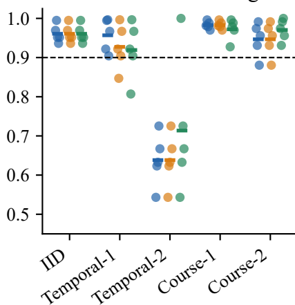
CatBoost Failure-class coverage
