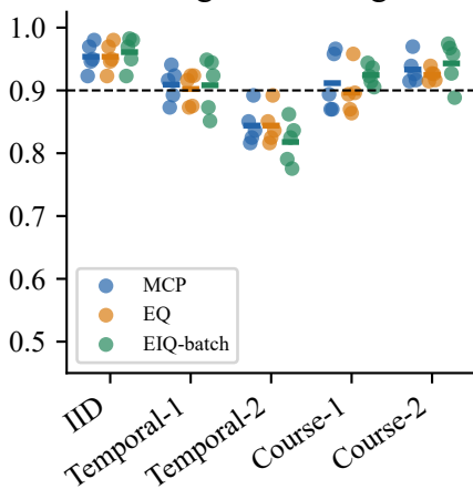
Logistic Marginal coverage
