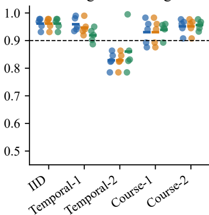
CatBoost Marginal coverage
