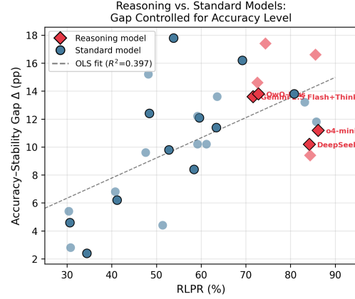
Figure 4: Accuracy–stability gap ( \Delta ) vs. RLPR for all 32 configurations. Reasoning models (diamonds) and standard models (circles) are shown against an OLS fit. Points below the line have smaller gaps than expected at their accuracy level.
