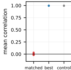
cross-seed agreement
