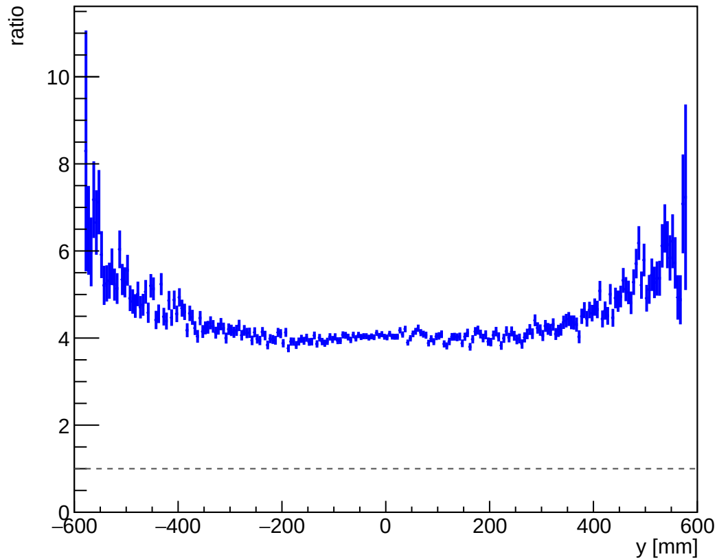
ratio of G4 stock / muon resampler: proton y position
