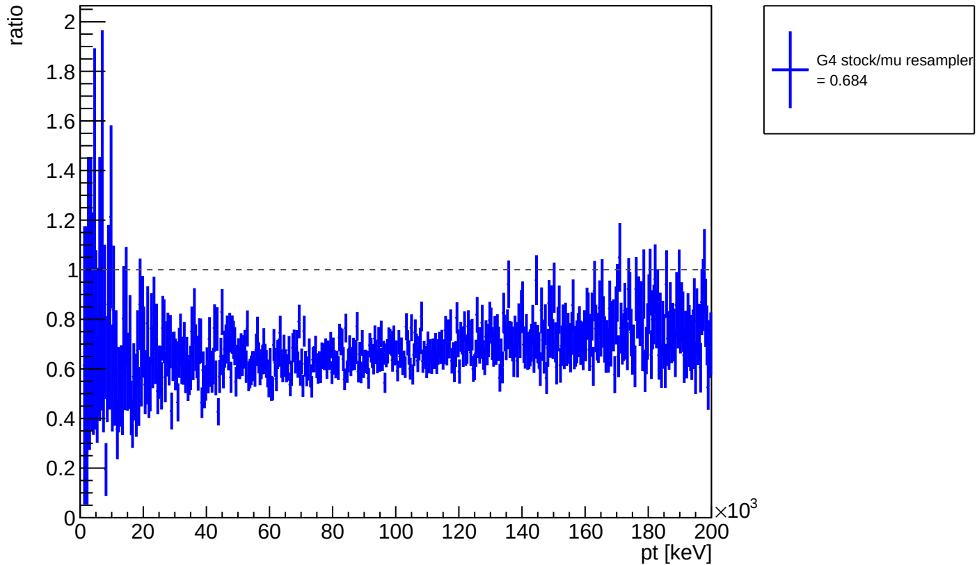
ratio of G4 stock / muon resampler: D transverse momentum pT
