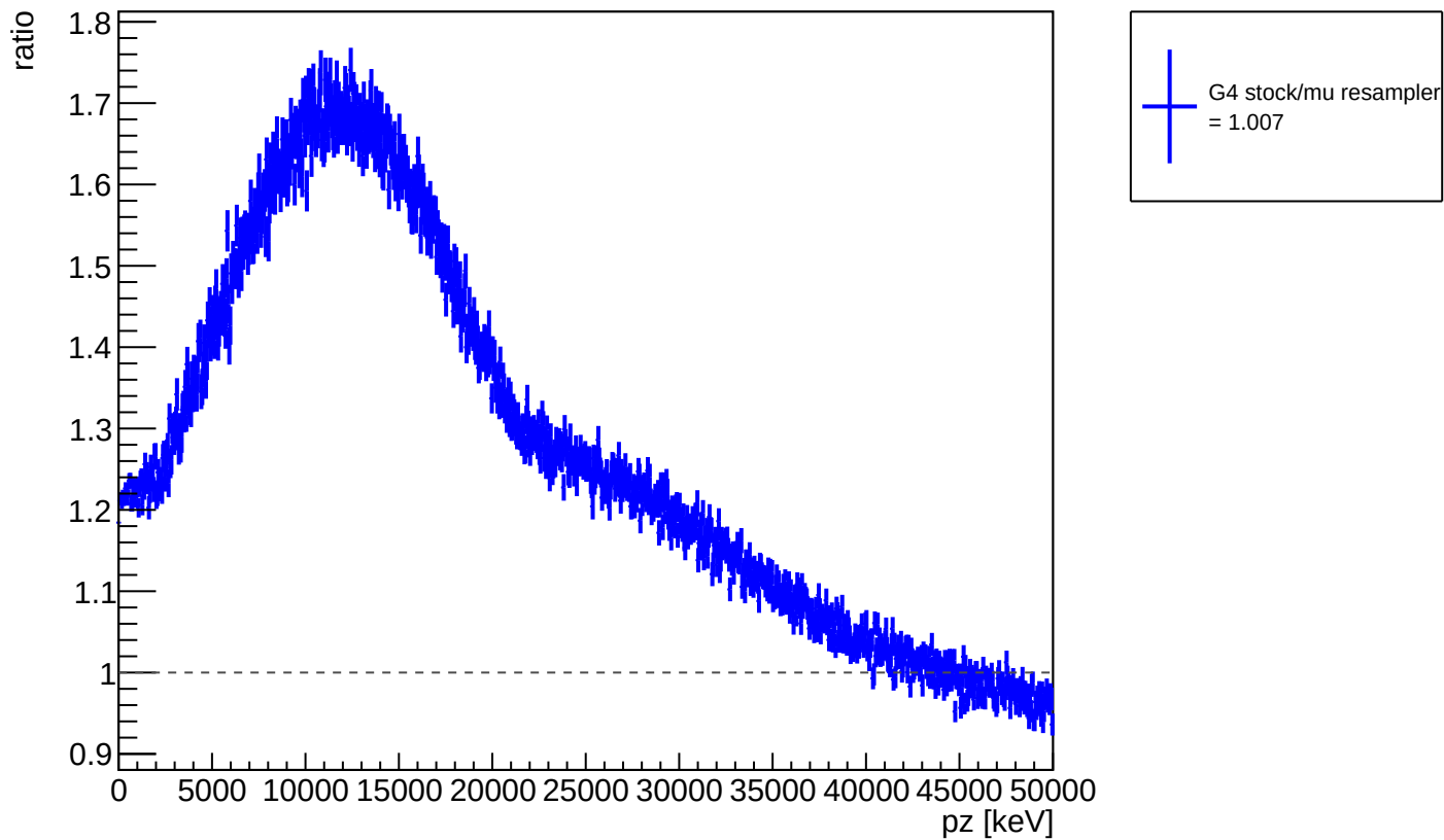
ratio of G4 stock / muon resampler: neutron momentum pz
