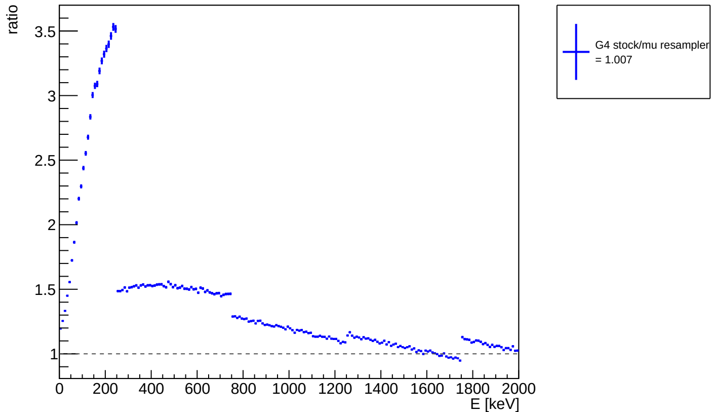
ratio of G4 stock / muon resampler: neutron kin. energy zoomed
