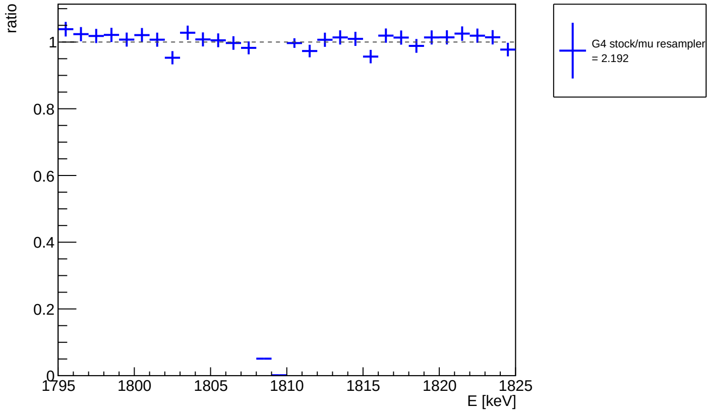
ratio of G4 stock / muon resampler: photon E (1795-1825 keV)
