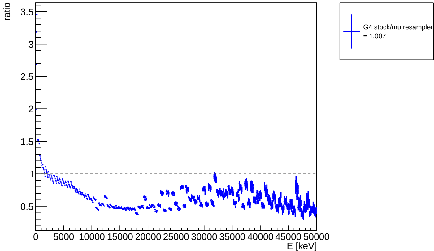
ratio of G4 stock / muon resampler: neutron kin. energy
