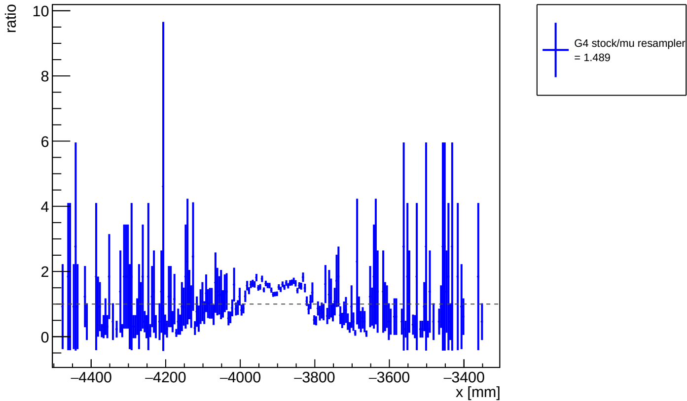
ratio of G4 stock / muon resampler: positron x position
