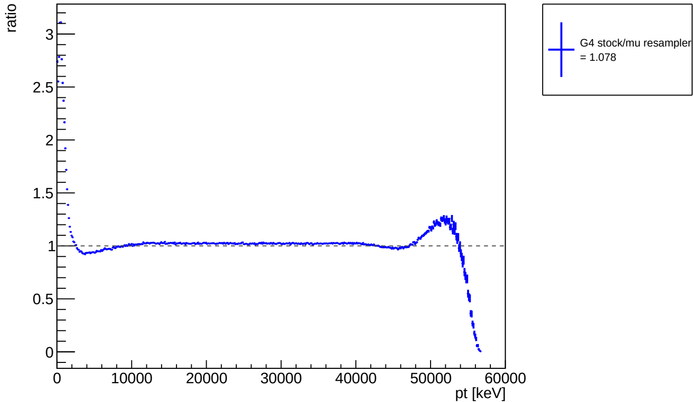
ratio of G4 stock / muon resampler: electron transverse momentum pT
