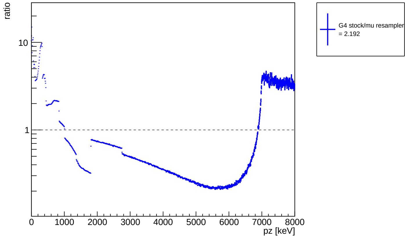
ratio of G4 stock / muon resampler: photon momentum pz
