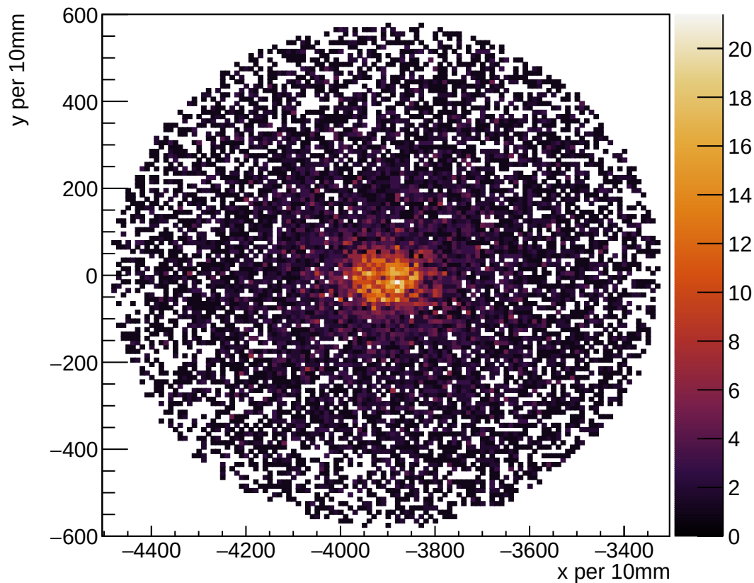
Stock G4: T y vs x
