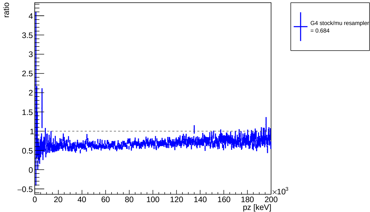
ratio of G4 stock / muon resampler: D momentum pz
