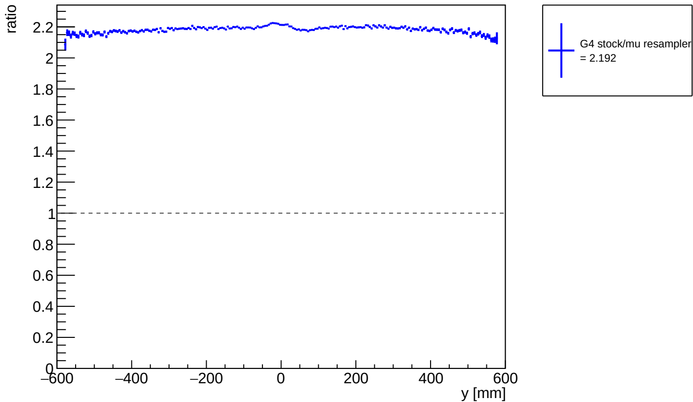
ratio of G4 stock / muon resampler: photon y position
