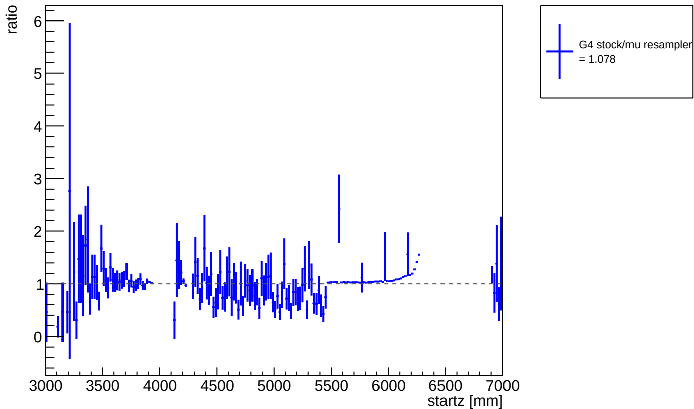
ratio of G4 stock / muon resampler: electron start z
