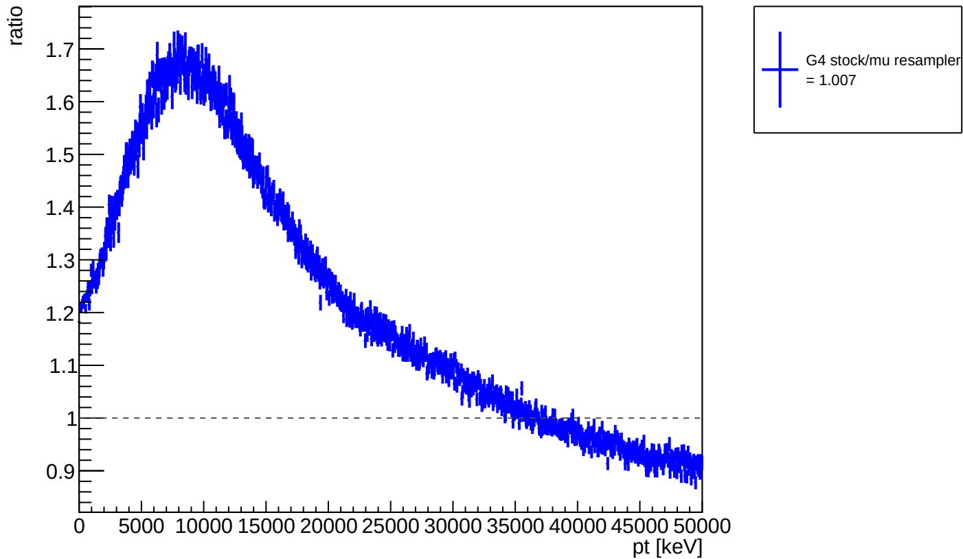
ratio of G4 stock / muon resampler: neutron transverse momentum pT
