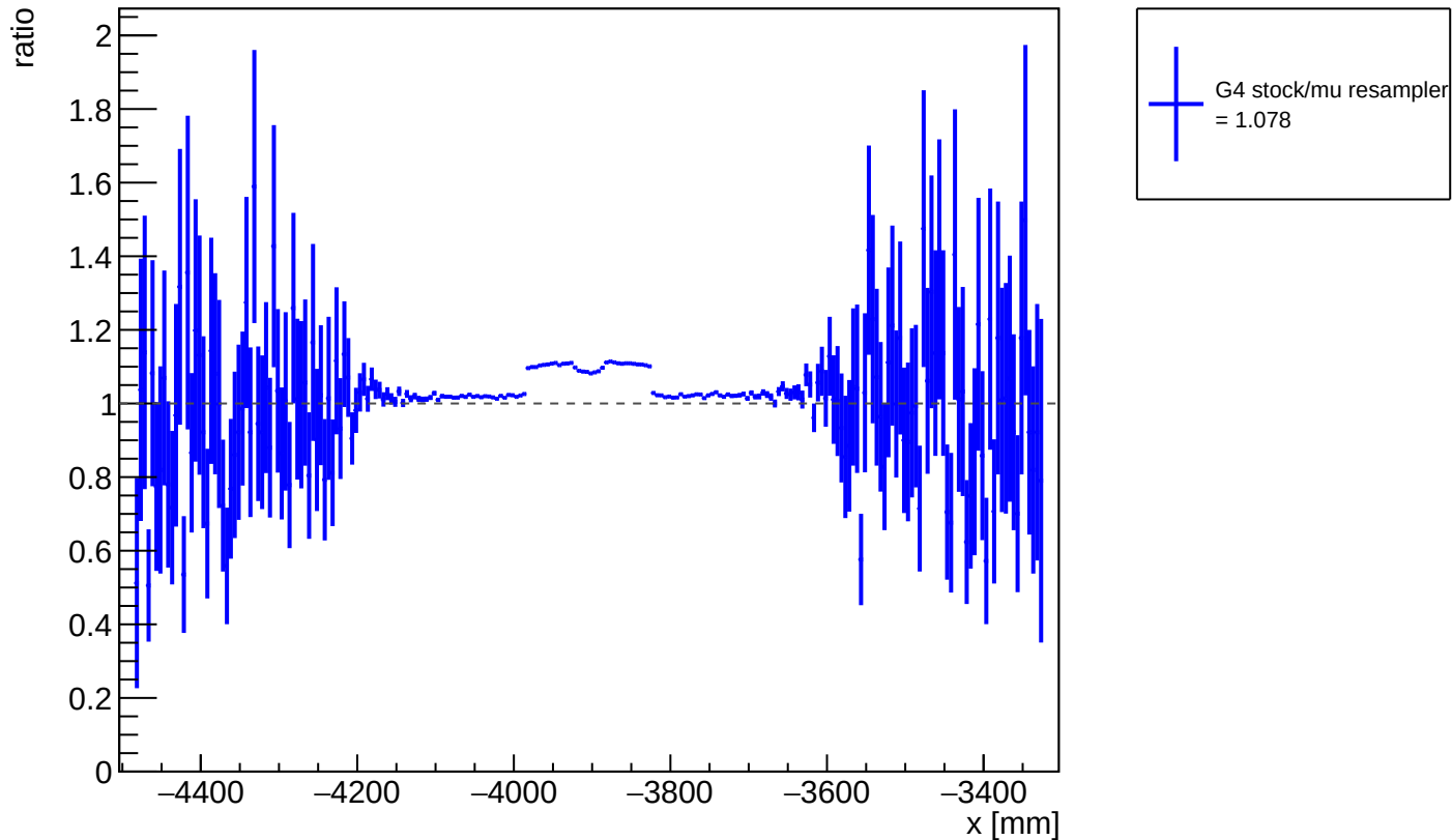
ratio of G4 stock / muon resampler: electron x position
