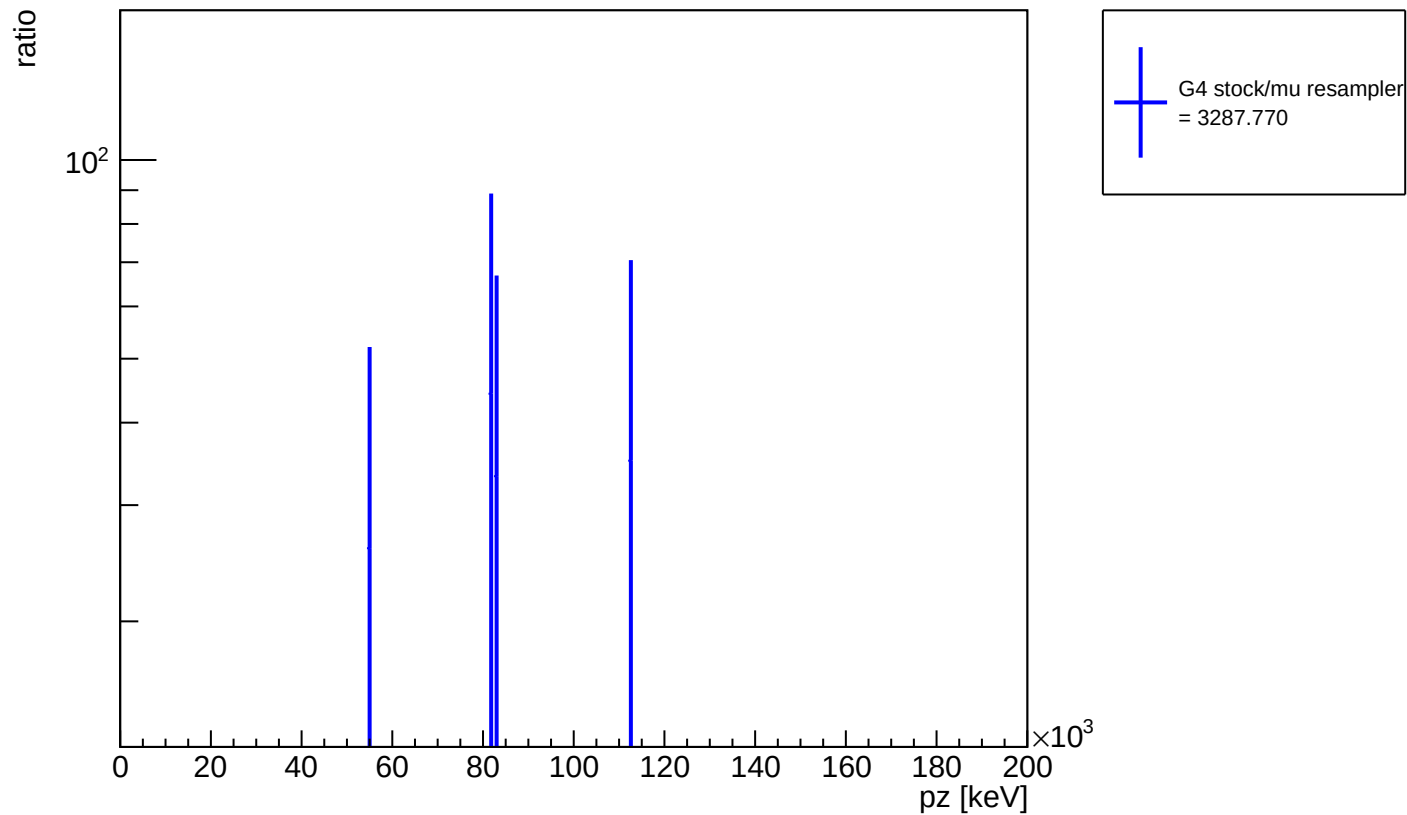
ratio of G4 stock / muon resampler: T momentum pz
