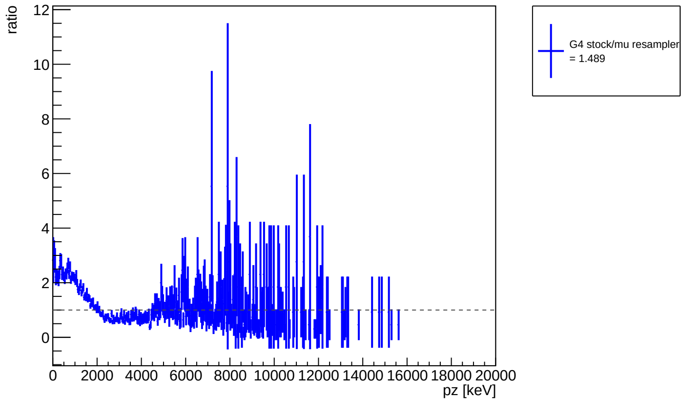
ratio of G4 stock / muon resampler: positron momentum pz
