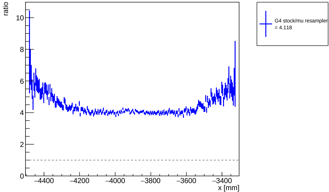
ratio of G4 stock / muon resampler: proton x position
