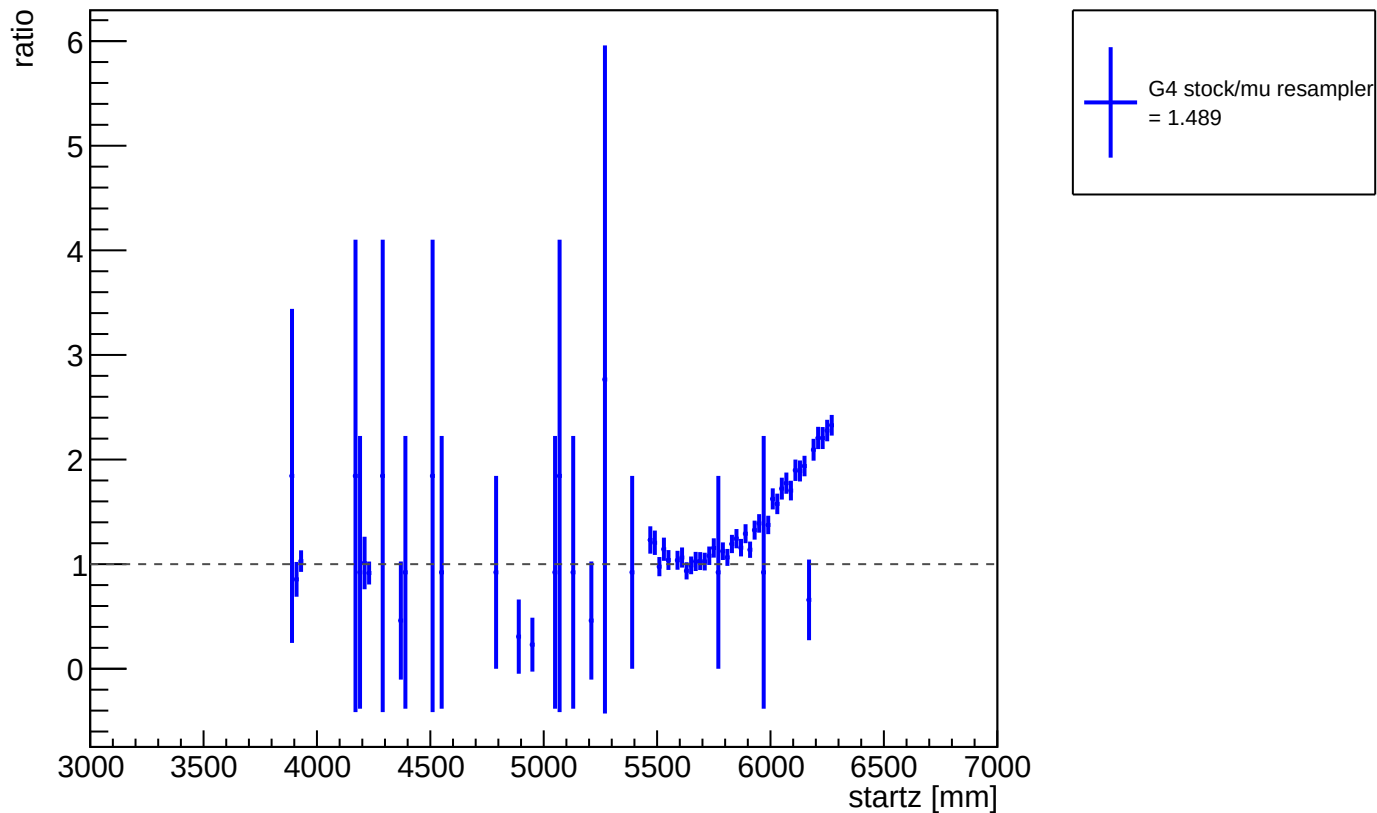
ratio of G4 stock / muon resampler: positron start z
