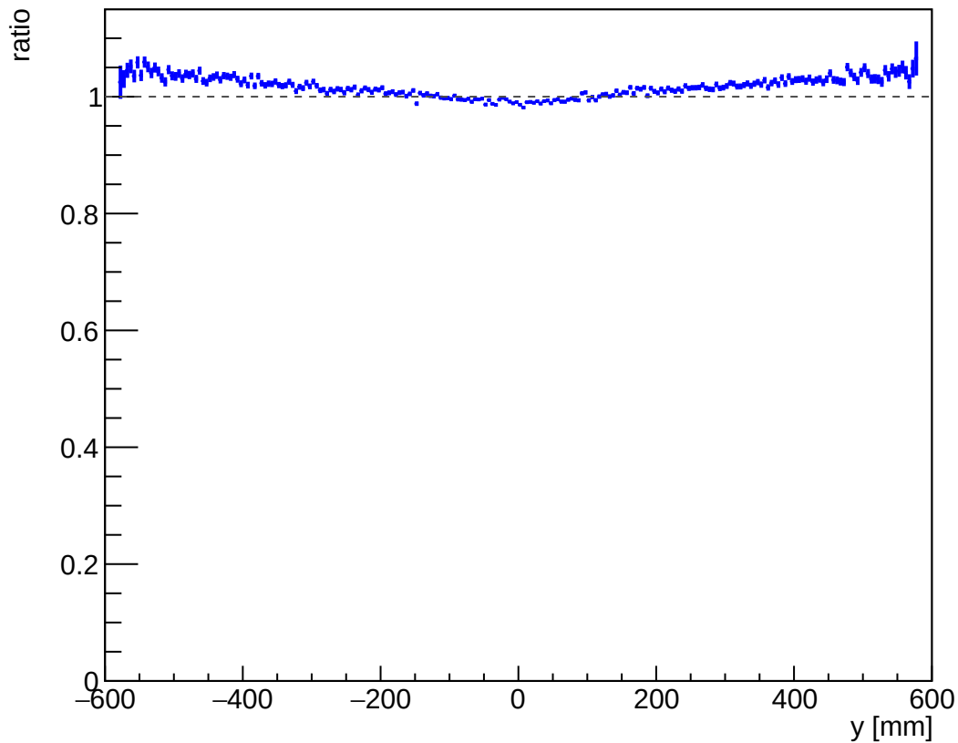
ratio of G4 stock / muon resampler: neutron y position
