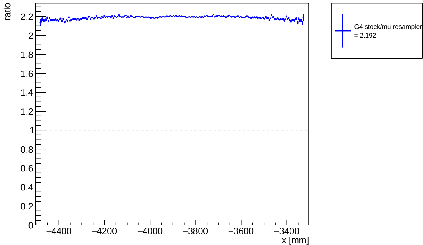
ratio of G4 stock / muon resampler: photon x position
