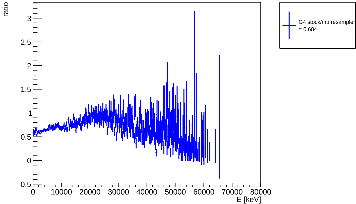
ratio of G4 stock / muon resampler: D kin. energy
