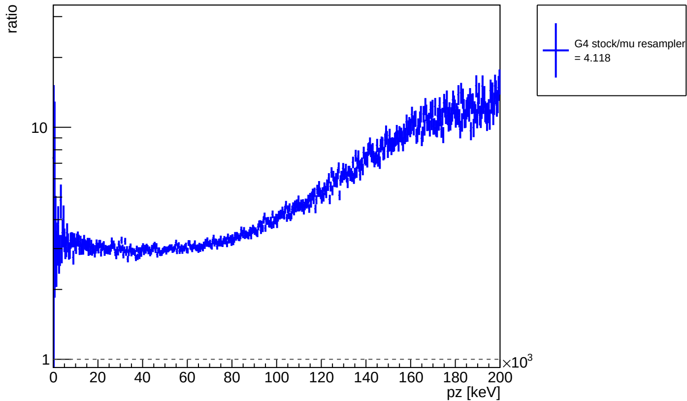
ratio of G4 stock / muon resampler: proton momentum pz
