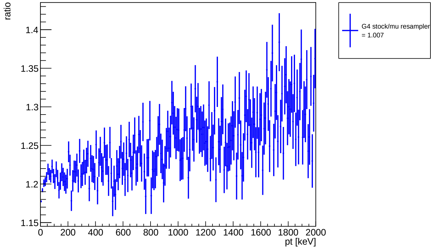
ratio of G4 stock / muon resampler: neutron transverse momentum pT zoomed
