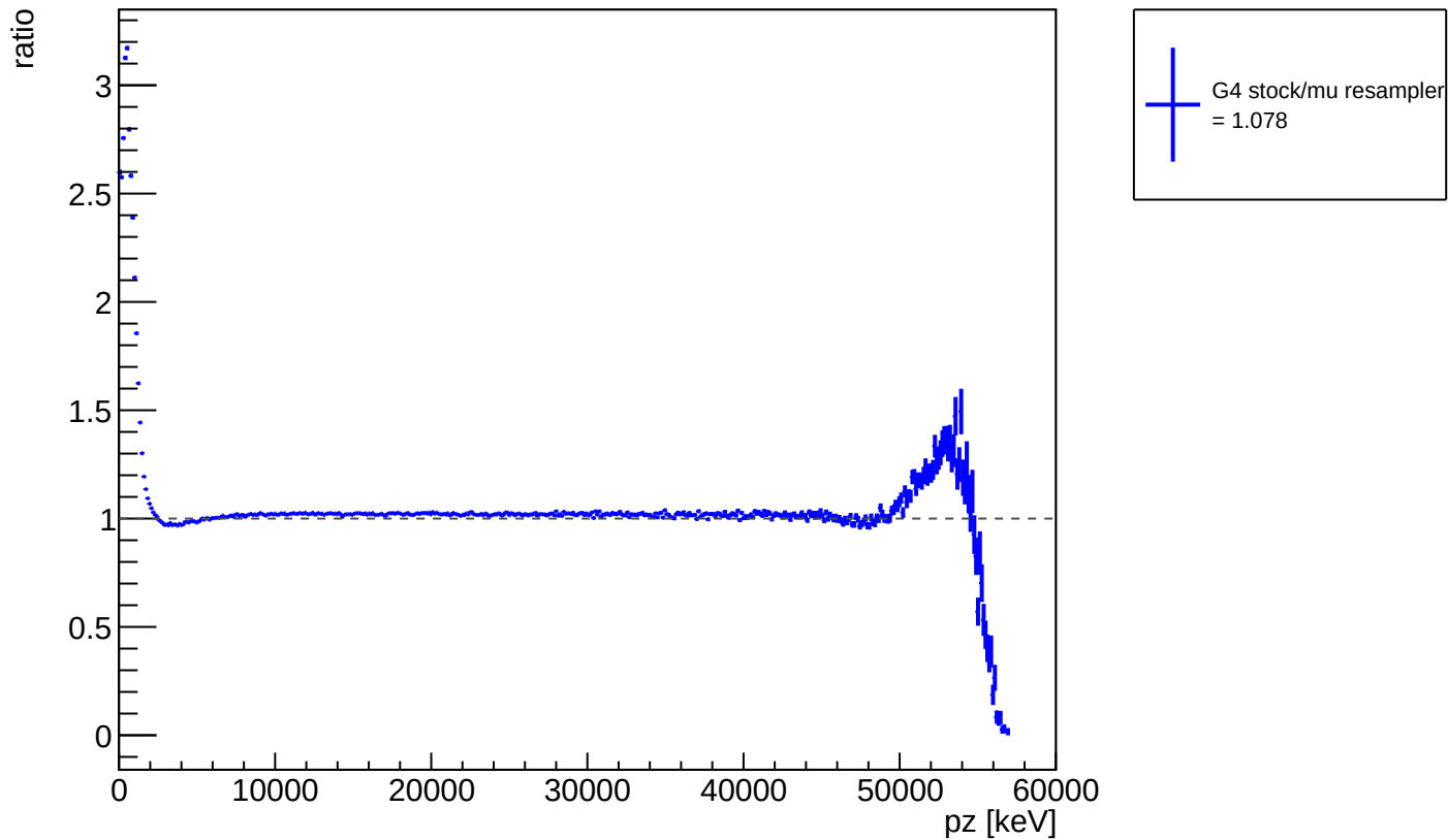
ratio of G4 stock / muon resampler: electron momentum pz
