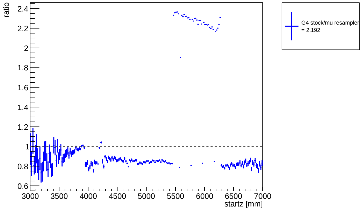
ratio of G4 stock / muon resampler: photon start z
