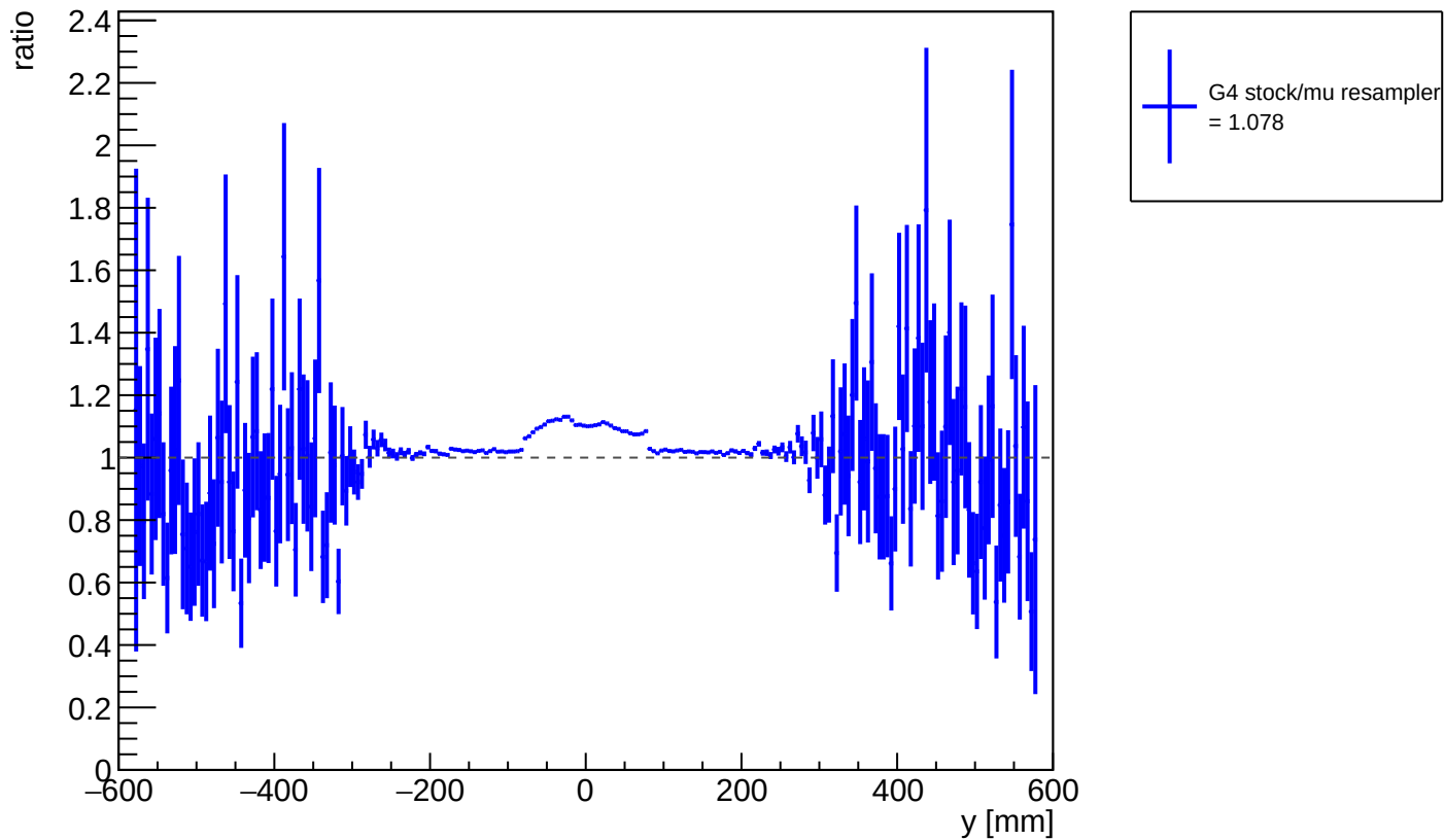
ratio of G4 stock / muon resampler: electron y position
