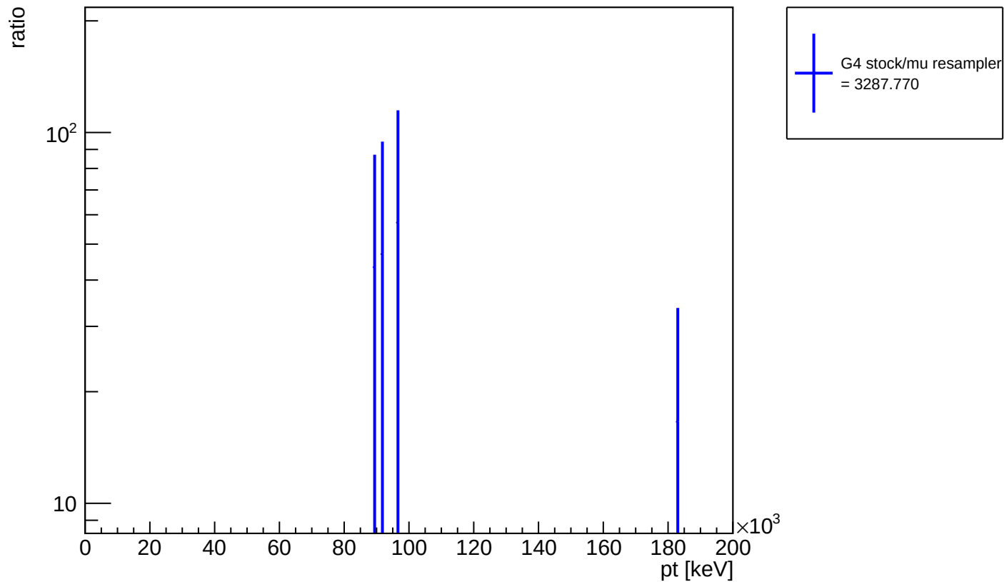
ratio of G4 stock / muon resampler: T transverse momentum pT
