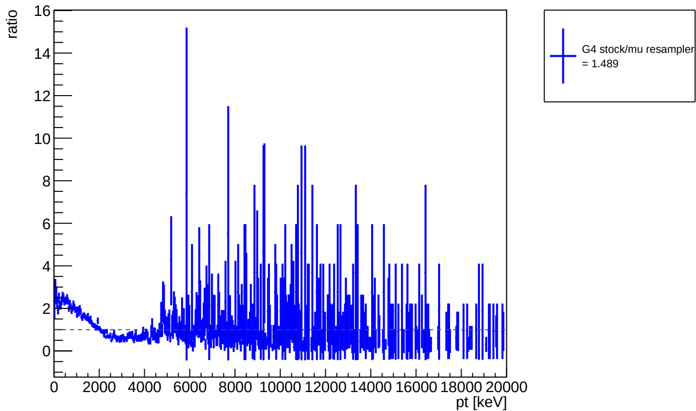
ratio of G4 stock / muon resampler: positron transverse momentum pT
