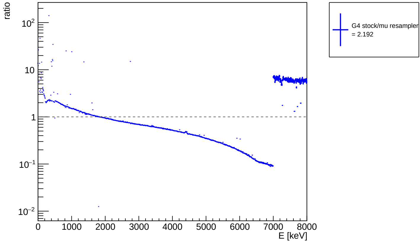
ratio of G4 stock / muon resampler: photon kin. energy
