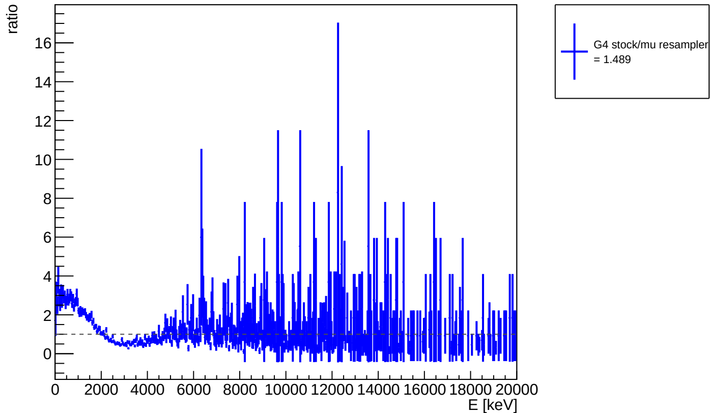
ratio of G4 stock / muon resampler: positron kin. energy
