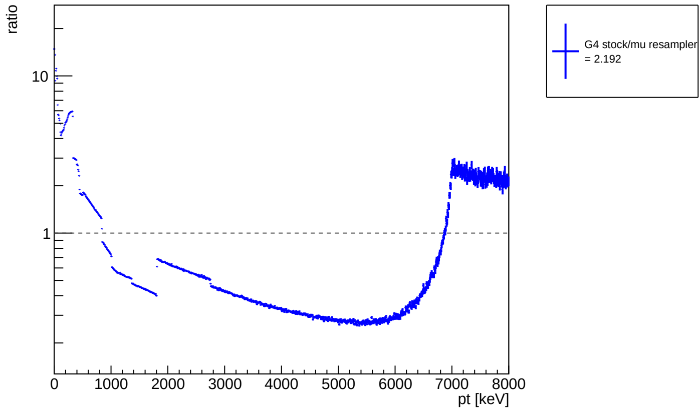
ratio of G4 stock / muon resampler: photon transverse momentum pT
