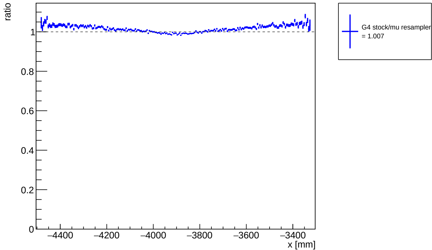
ratio of G4 stock / muon resampler: neutron x position
