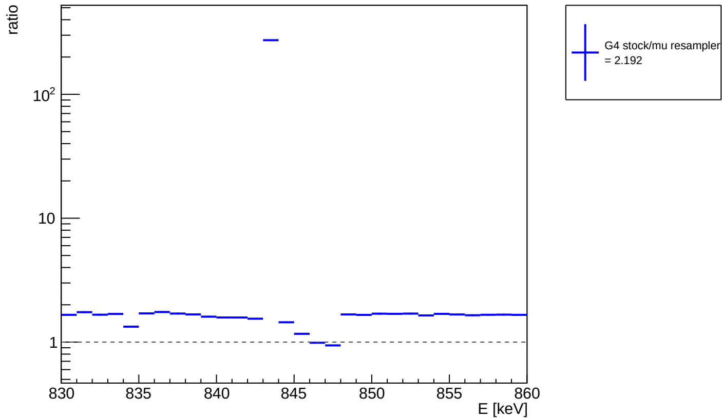
ratio of G4 stock / muon resampler: photon E (830-860 keV)
