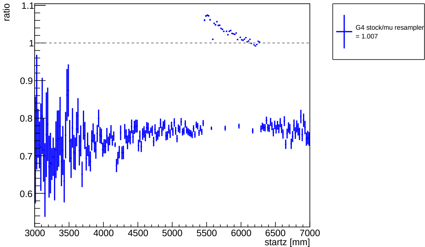
ratio of G4 stock / muon resampler: neutron start z
