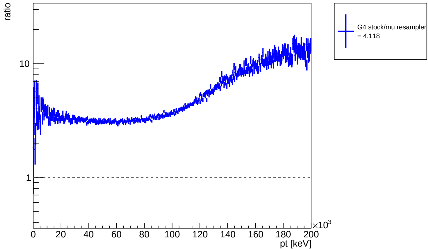
ratio of G4 stock / muon resampler: proton transverse momentum pT
