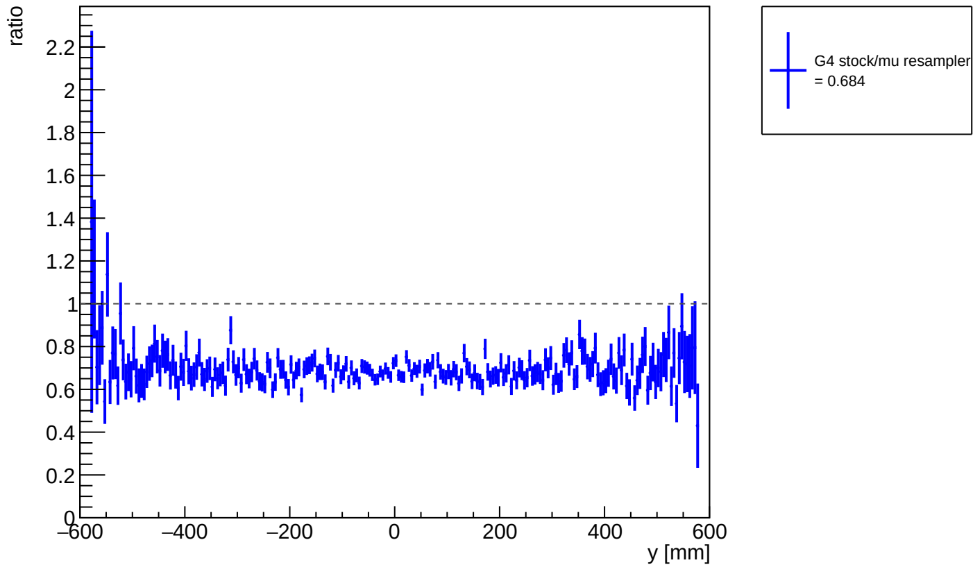
ratio of G4 stock / muon resampler: D y position
