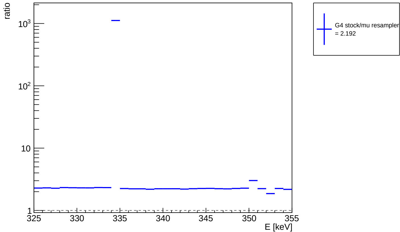
ratio of G4 stock / muon resampler: photon E (325-355 keV)
