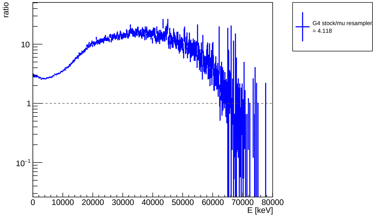
ratio of G4 stock / muon resampler: proton kin. energy
