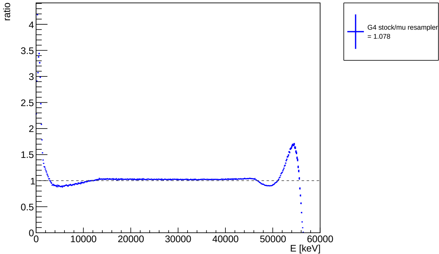
ratio of G4 stock / muon resampler: electron kin. energy
