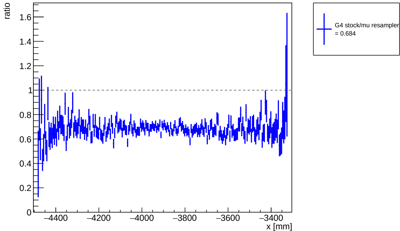
ratio of G4 stock / muon resampler: D x position
