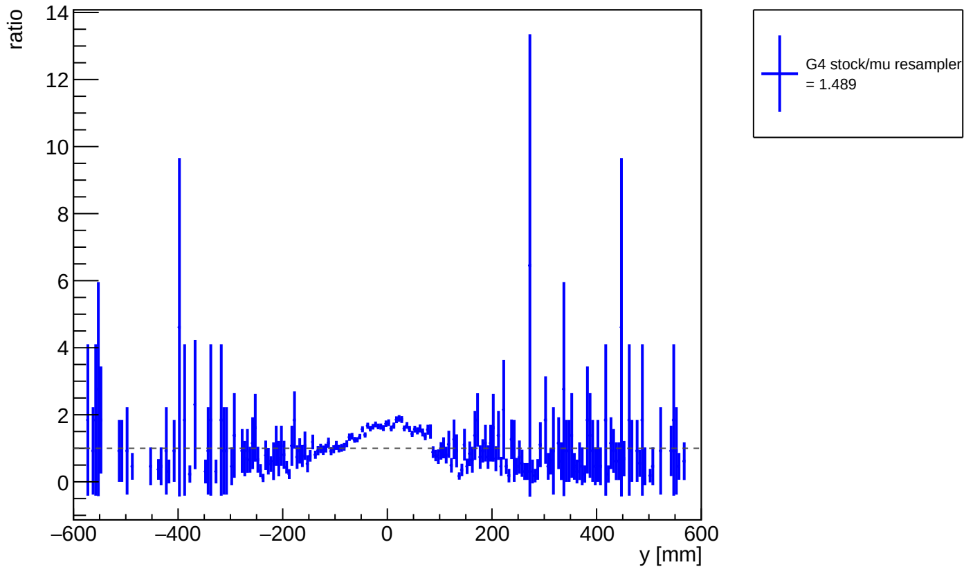
ratio of G4 stock / muon resampler: positron y position
