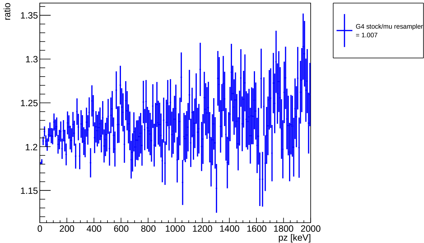
ratio of G4 stock / muon resampler: neutron momentum pz zoomed
