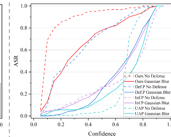
Gaussian blur
