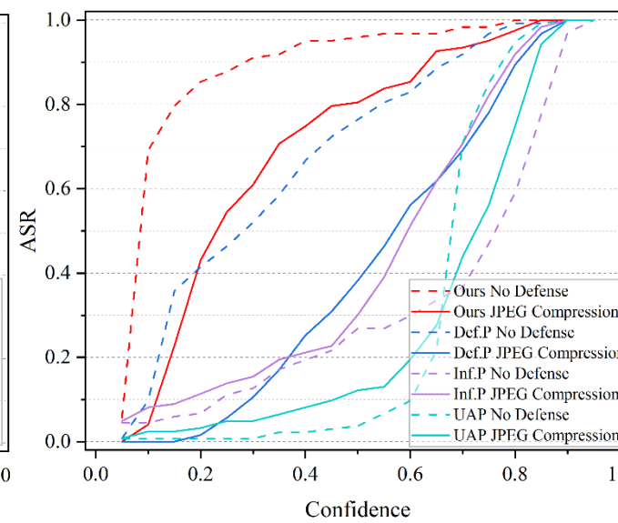
JPEG Compression
