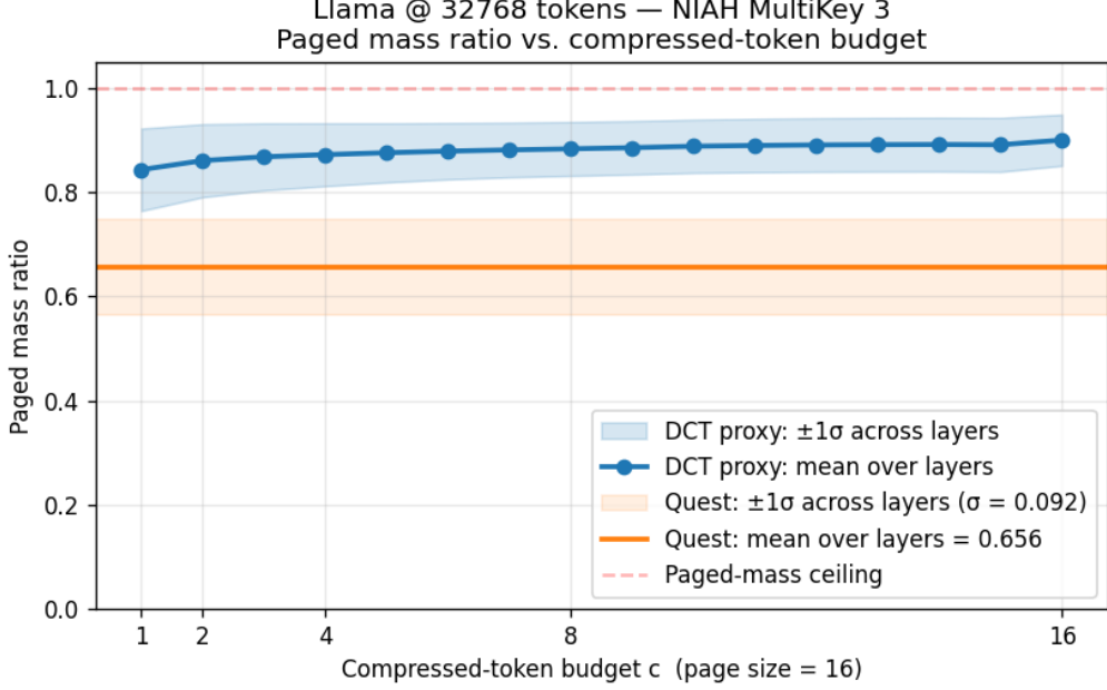
Figure 6.1: Paged attention-mass recall (Eq. (6.1)) on a RULER NIAH-MultiKey 3 trace at L = 32,768 with Llama-3.1-8B-Instruct, page size P=16 , selected-token budget B \cdot P = 2,048 . The DCT-lowpass-IDCT proxy of Section 3.3 (blue) already routes \approx 84\% of the dense softmax mass to its selected pages at the most aggressive setting c=1 (one proxy token per 16 keys), and the curve climbs gently to \approx 90\% at c=16 before saturating; the per-channel min/max scorer of Quest (orange) covers only 65.6% of the mass at the same selected-token budget, regardless of c . Shaded bands are \pm 1\sigma across transformer layers.
