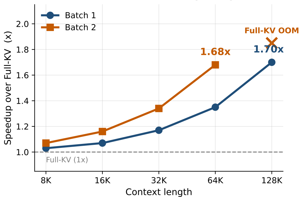
End-to-end decode speedup
