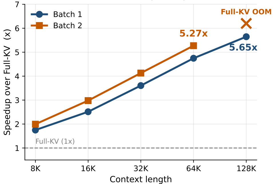
Attention speedup
