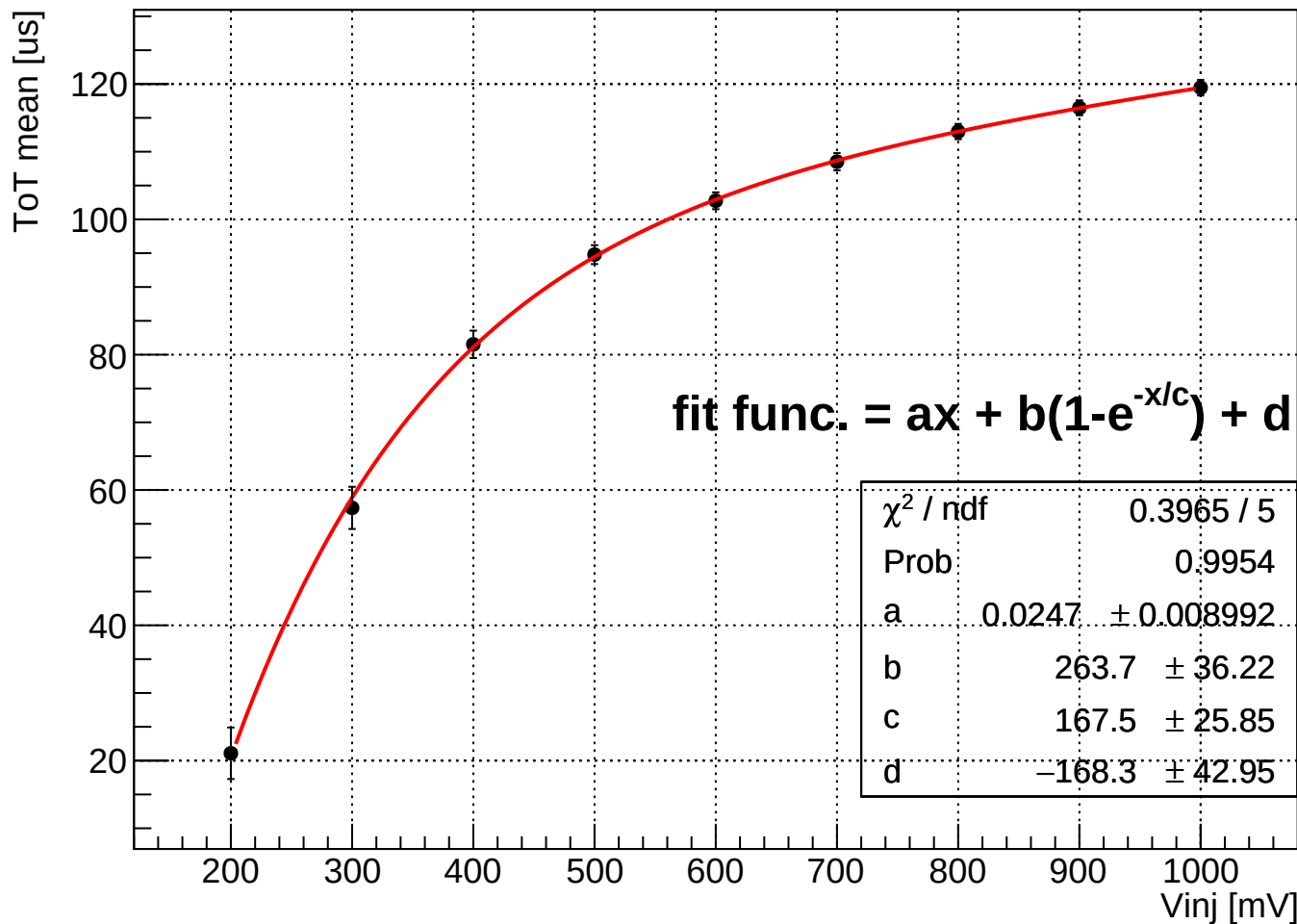
Injection Voltage vs ToT mean from gaussian fitting
