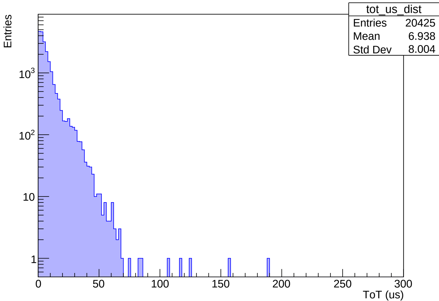
ToT Distribution for row=3, col=9
