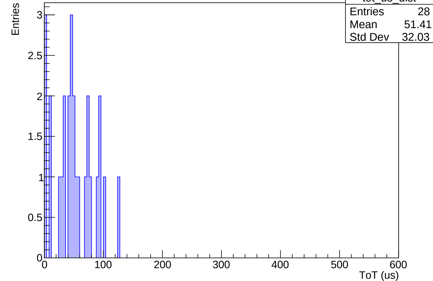
ToT Distribution for row=8, col=8
