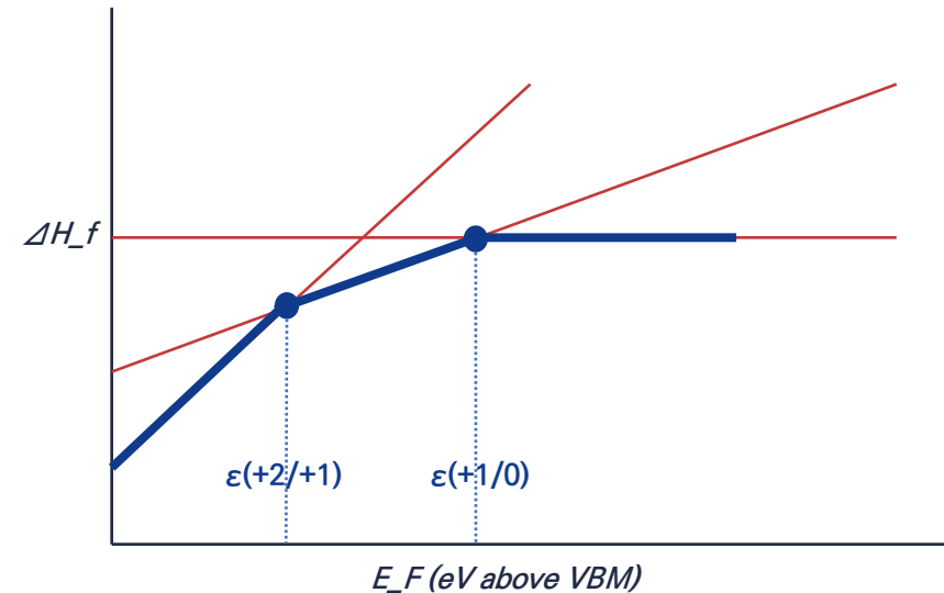
Charge Transition Level
