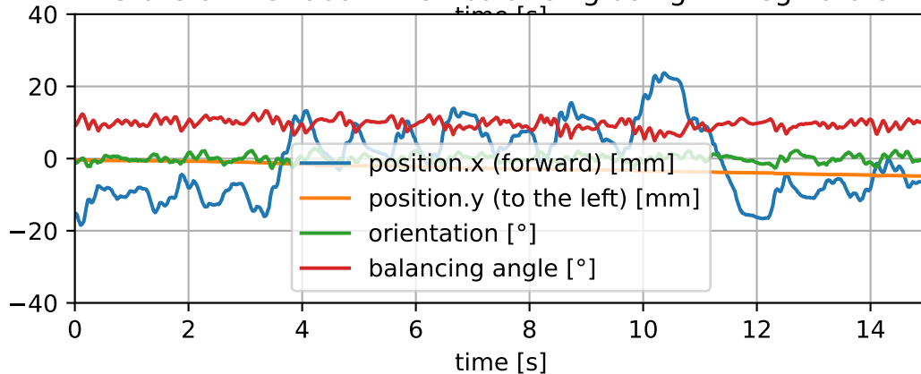
State of the robot when balancing using LinRegMotors
