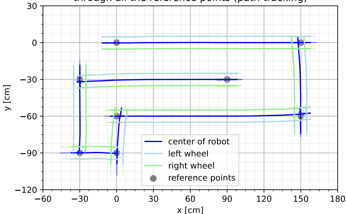
Position of the robot (enc. only) as it travels through all the reference points (path tracking)
