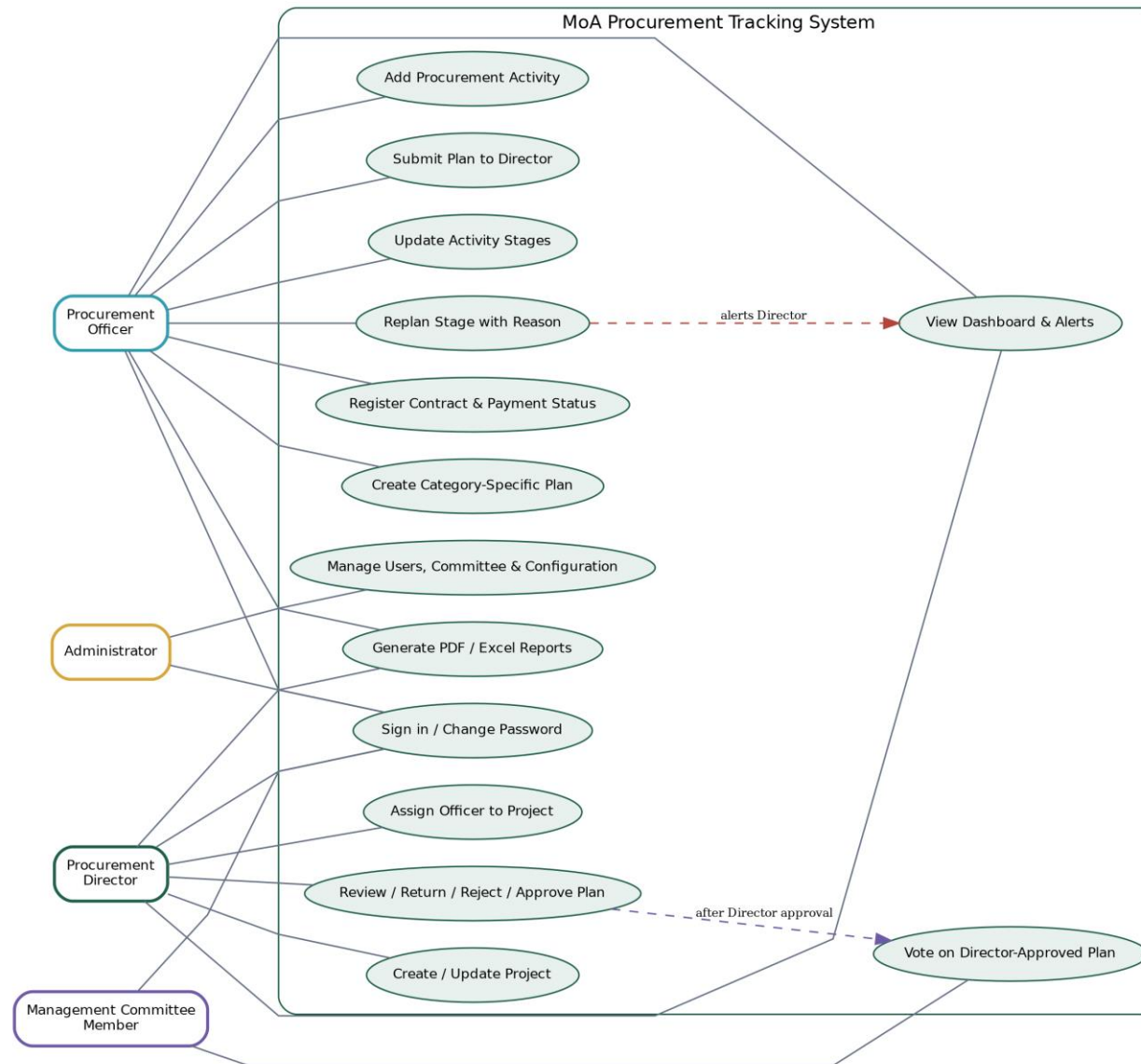
Figure 2. Use case diagram for the four confirmed actors.
