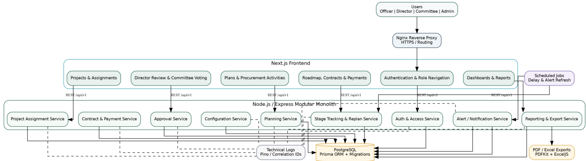
Figure 1. Updated component diagram - document storage and audit-history components are removed; project assignment and approval components are added.
