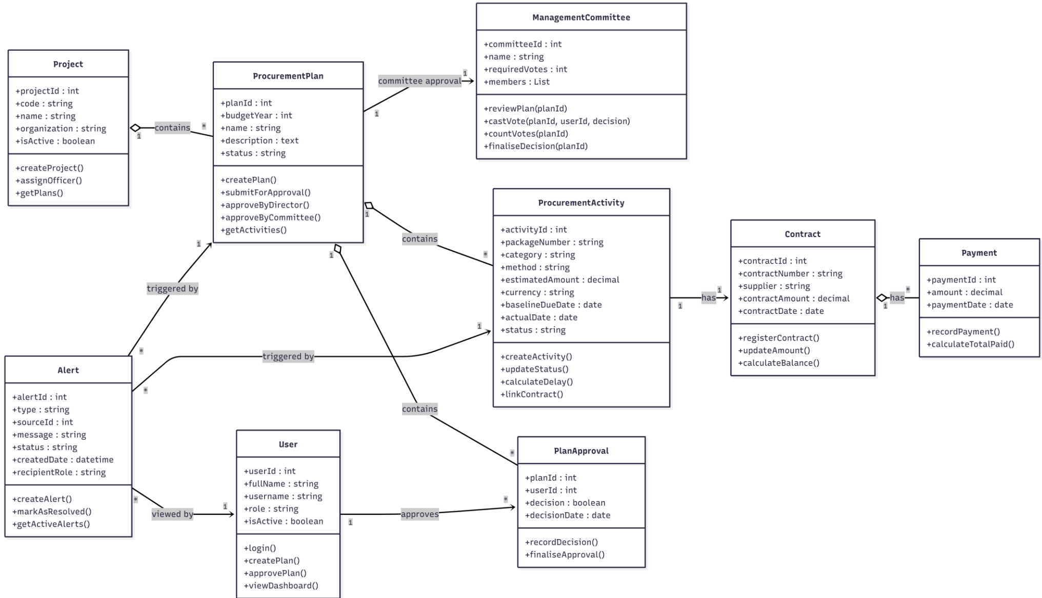
Figure 5. Updated domain class diagram.
