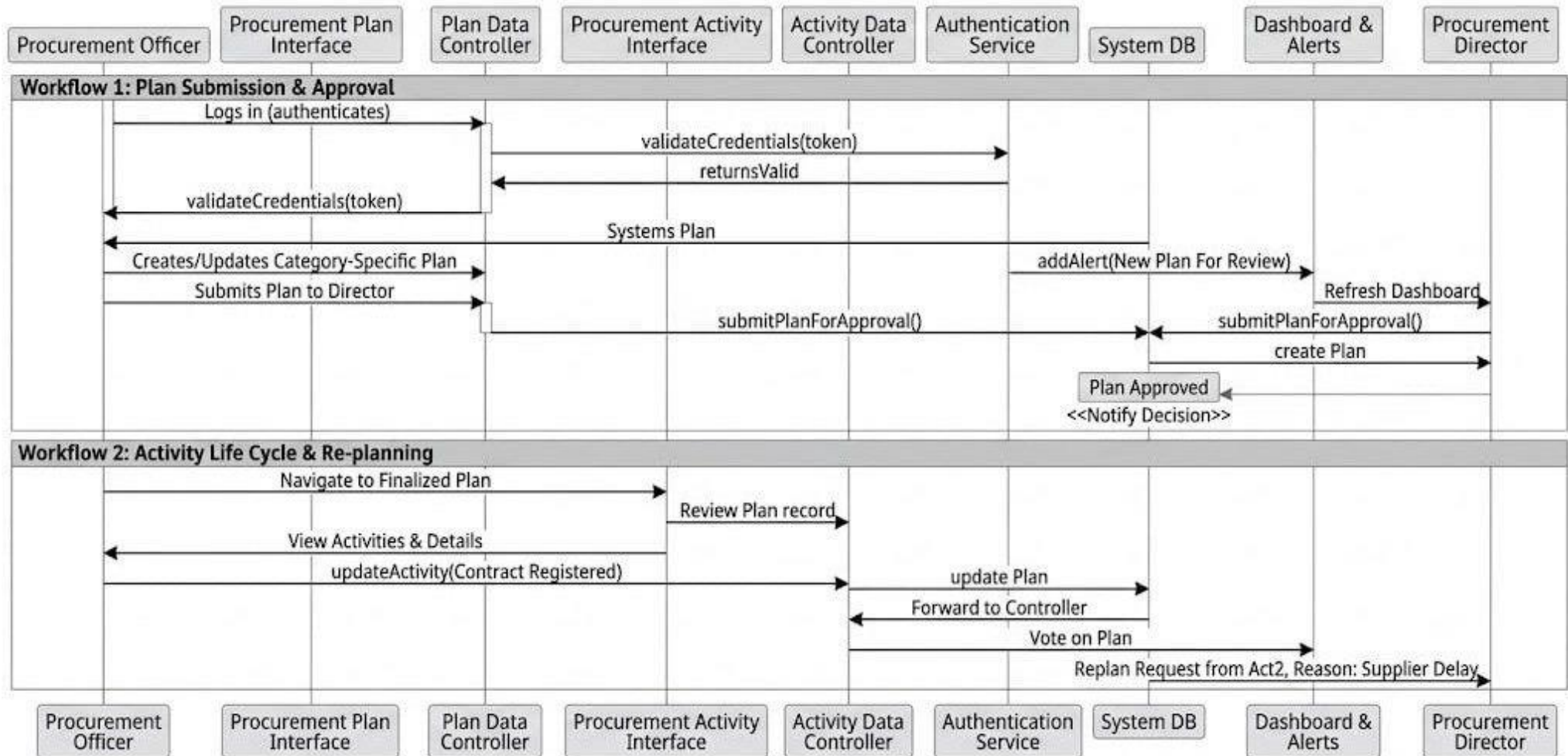
Figure 4. Plan submission, Director approval and committee voting sequence.
