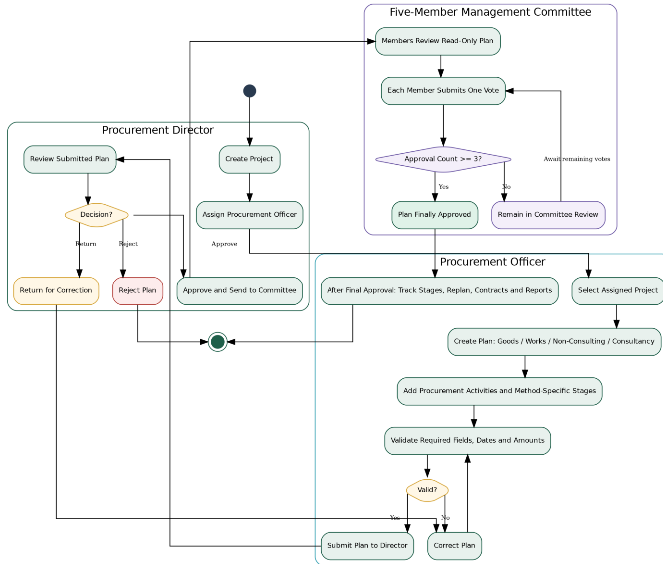
Figure 3. Plan creation and approval activity diagram.
