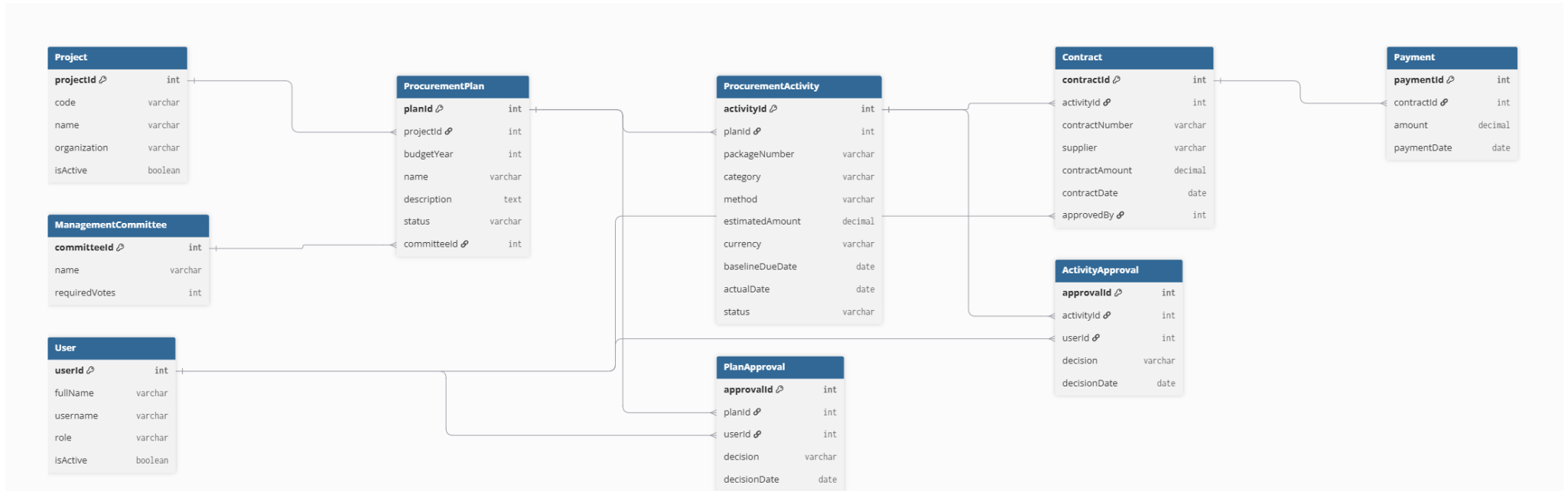
Figure 6. Updated ERD including project assignments and two-level plan approval; document and audit-history entities are removed.
