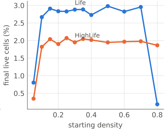
Density of the settled 'ash'
