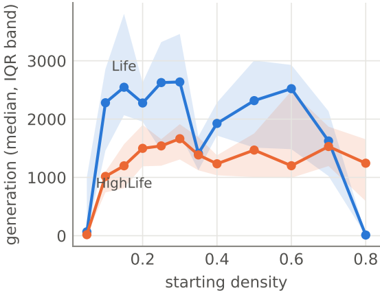
Generation of first repeated state
