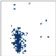
complex, d=0.35
