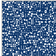
oscillating, d=0.20
