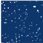
stable, d=0.20
