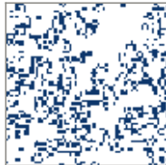
chaotic, d=0.20
