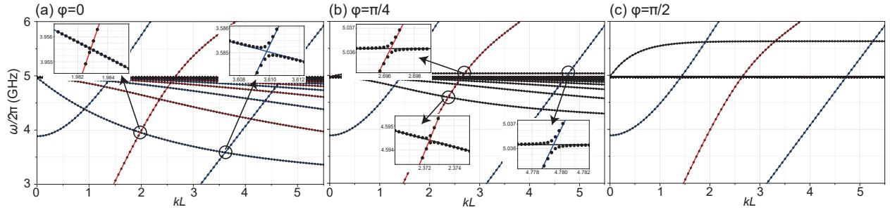
Figure 2. Dispersion curves of the coupled waves. Red and blue curves represent modes with C_{2x} eigenvalues +1 and -1 , respectively. Black curves represent magnetostatic modes that are not eigenstates of the C_{2x} operator. Markers show the dispersion of the coupled waves obtained from numerical calculations. The external magnetic field is applied (a) parallel to the propagation direction, \mathbf{H}_0 \parallel \mathbf{k} ( \varphi = 0 ), (b) at \varphi = \pi/4 , and (c) perpendicular to the propagation direction, \mathbf{H}_0 \perp \mathbf{k} ( \varphi = \pi/2 ). Insets show magnified views of representative band crossings. In (a), \varphi = 0 , anticrossings appear between BVW and Lamb modes only when they have the same C_{2x} eigenvalue (same color). When the C_{2x} symmetry of the system is broken (b), both the magnetostatic surface mode and the BVW couple to Lamb modes. The bottom-center inset of panel (b) shows the hybridization between the lowest-frequency BVW mode and the first Lamb wave mode.
