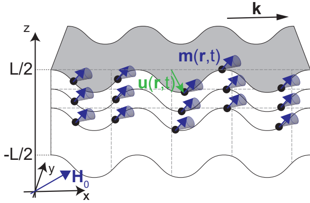
Figure 1. Schematic illustration of the system under consideration. A ferromagnetic thin film with thickness L in the z direction and infinite extent in the x and y directions is considered. Magnetic moments at each lattice point precess around an axis parallel to the in-plane external magnetic field \mathbf{H}_0 . The elastic wave changes the positions of the magnetic moments and their separations, resulting in a modification of the dipolar interaction among them.
