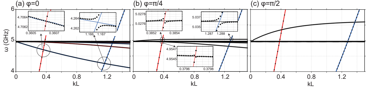
Figure 2. Dispersion curves of the coupled waves. Red and blue curves represent symmetric and antisymmetric modes of the uncoupled waves, including magnetostatic backward volume waves (BVWs) and Lamb waves, while black curves represent magnetostatic modes that are neither symmetric nor antisymmetric. Black dots Markers show the dispersion of the coupled waves obtained from numerical calculations. The external magnetic field is applied (a) parallel to the propagation direction, \mathbf{H}_0 \parallel \mathbf{k} ( \varphi = 0 ), (b) at \varphi = \pi/4 , and (c) perpendicular to the propagation direction, \mathbf{H}_0 \perp \mathbf{k} ( \varphi = \pi/2 ). Insets show magnified views of representative band crossings. In (a) \varphi = 0 , anticrossings appear between BVW and Lamb modes only when they have the same C_{2x} eigenvalues (same color). When the C_{2x} symmetry of the system is broken (b), both the magnetostatic surface mode and the BVW couple to Lamb modes. The bottom-center inset of panel (b) shows the hybridization between the lowest-frequency backward volume wave mode and the first Lamb wave mode.
