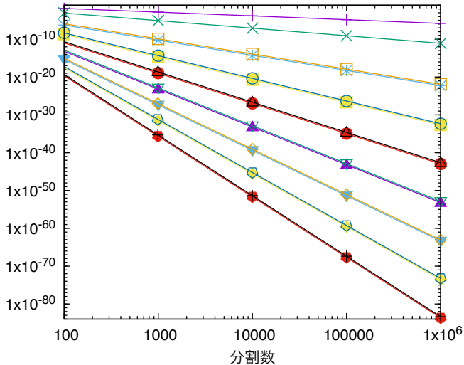
Simpson's rule
