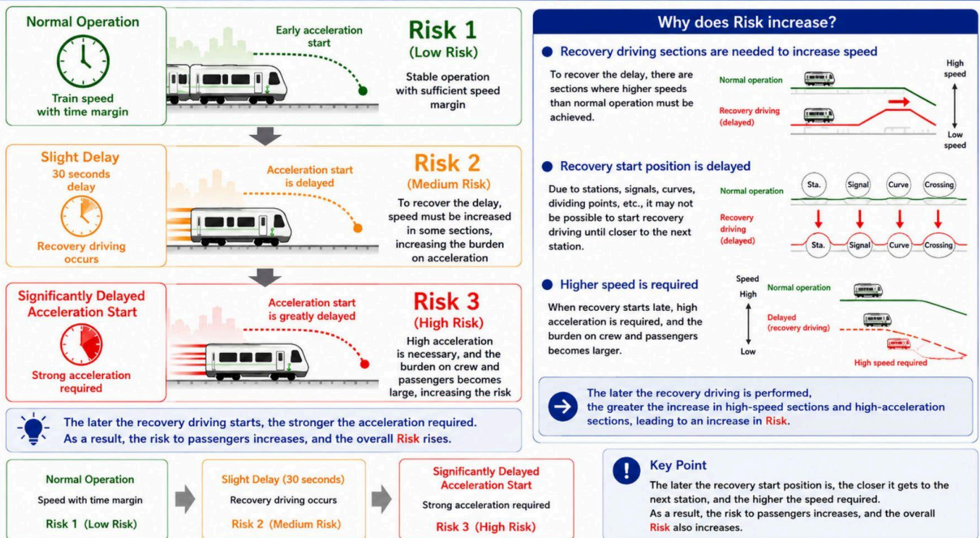
Fig. 6-1 Delayed Recovery Driving Model
