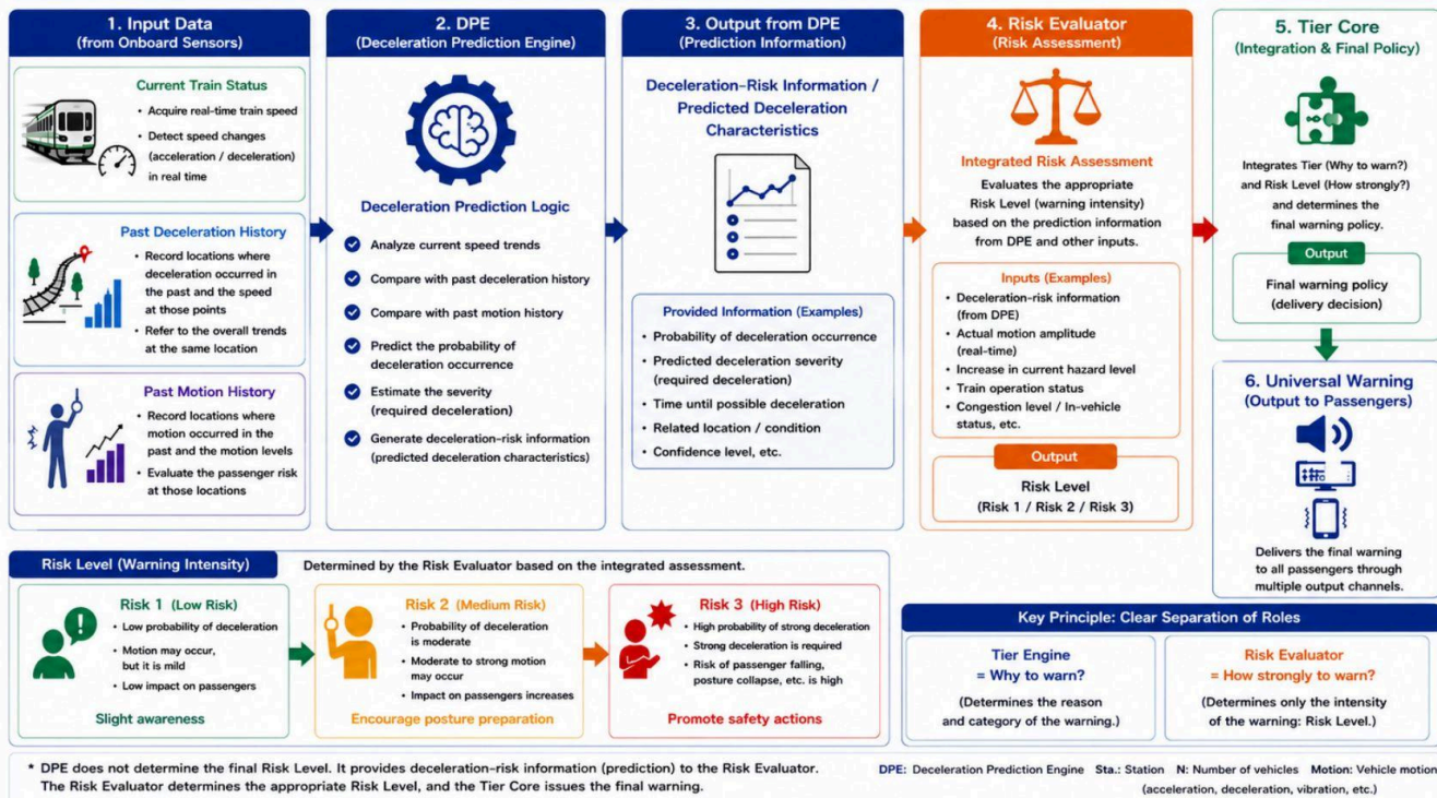
Fig. 6-2 Deceleration Warning Generation Diagram (DPE) [Revised]
