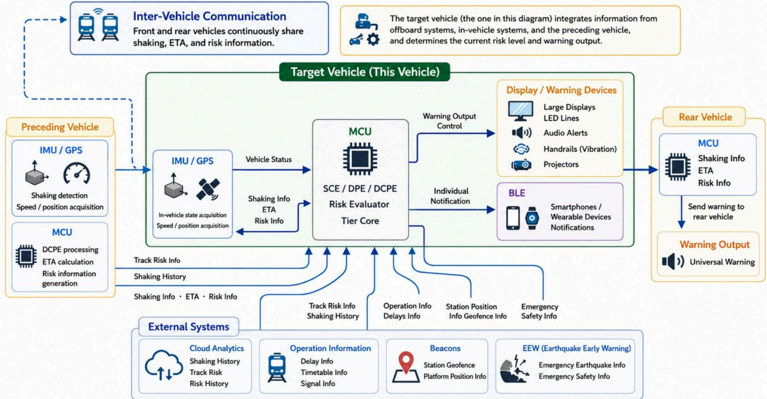
Fig. 3-3 URSAS 5.4 Onboard–Offboard Communication System
