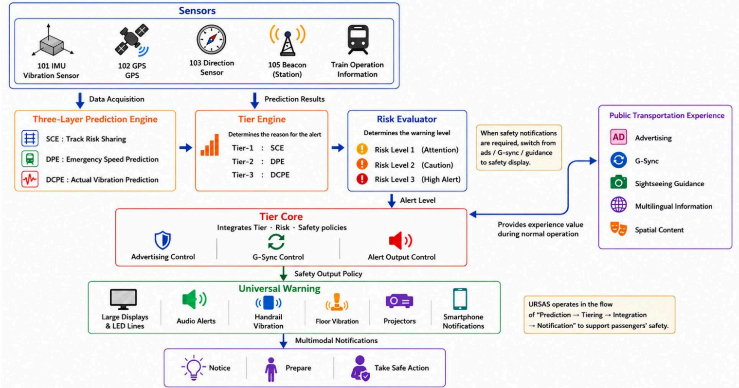
Fig. 3-1 URSAS 5.4 System Architecture (Overview)
