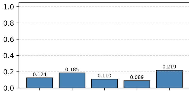
Recall
