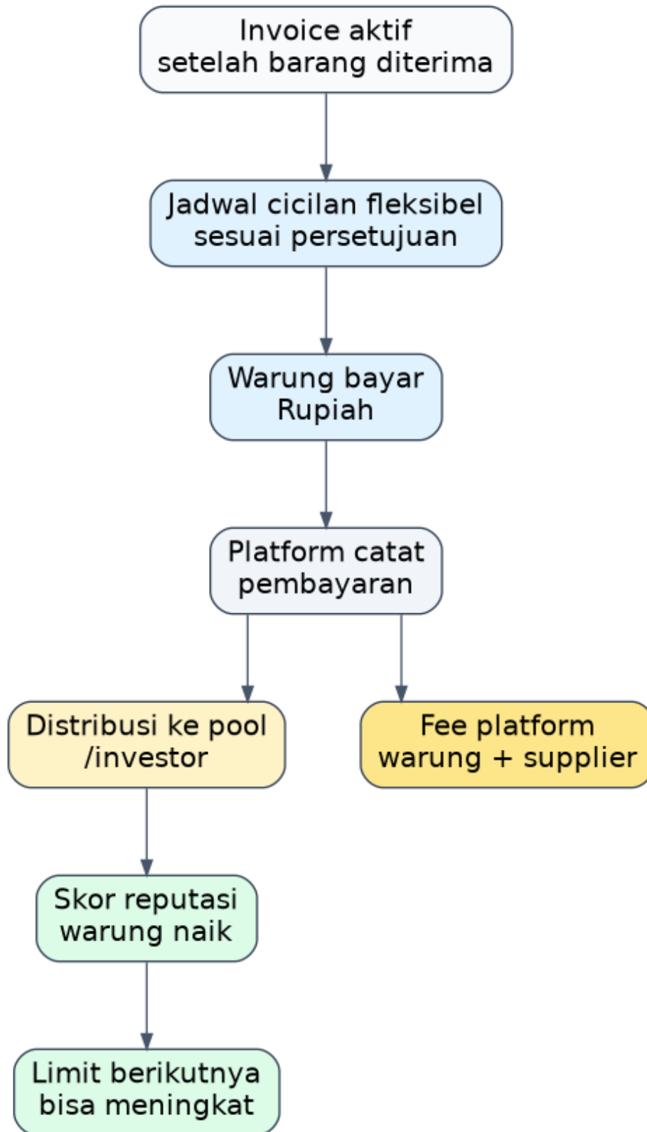
Gambar 4 - Activity Diagram Cicilan dan Repayment
