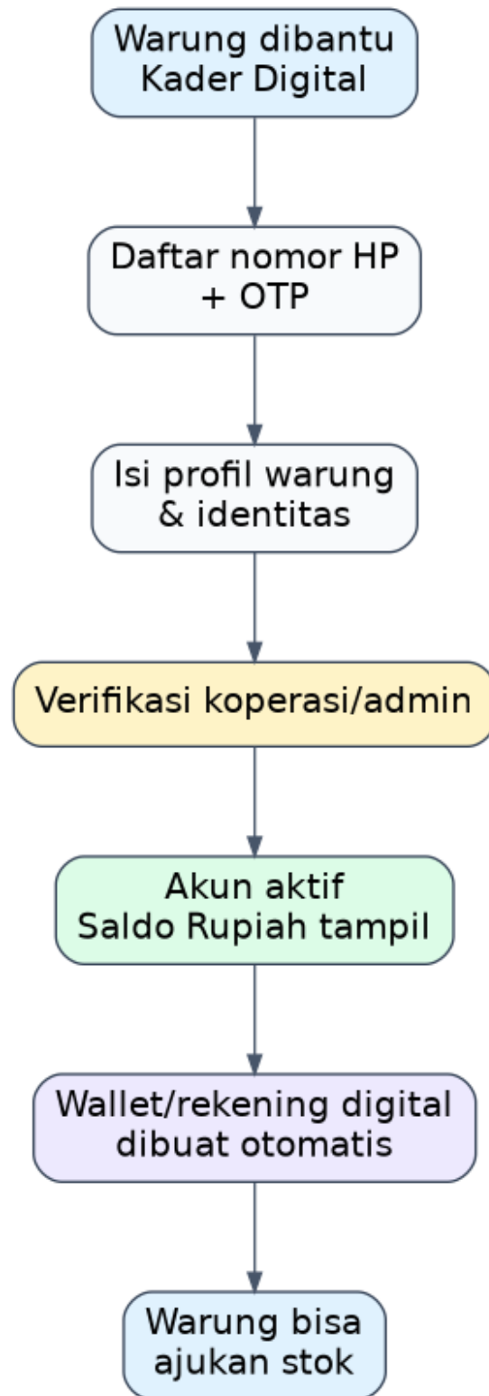
Gambar 2 - Activity Diagram Onboarding Warung
