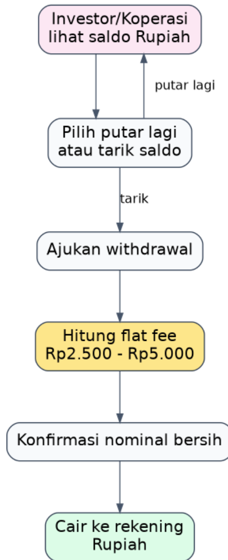
Gambar 5 - Activity Diagram Withdrawal Investor/Koperasi
