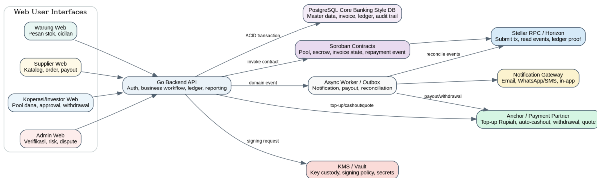
Gambar 2 - Arsitektur high-level website, Go backend, database, Stellar, Soroban, dan partner fiat
