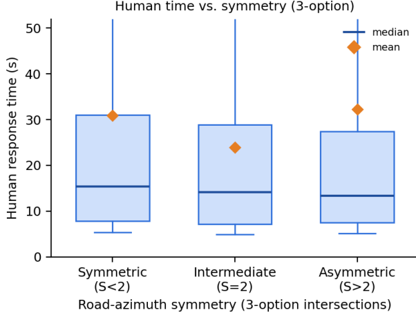
Figure 6. Human response time vs. road-azimuth symmetry (three-option intersections). Distribution of per-response times (engaged annotators who completed all 200 items) by symmetry level S (Eq. 2), holding candidate count fixed. Boxes show the interquartile range, whiskers the 10th–90th percentiles, the line the median, and the diamond the mean. The lower quartile is similar across all levels (a shared easy floor), but symmetric intersections ( S < 2 ) have a markedly longer upper tail (higher 75th/90th percentiles) than asymmetric ones ( S > 2 ): structural symmetry raises the ceiling on difficulty without determining it.
