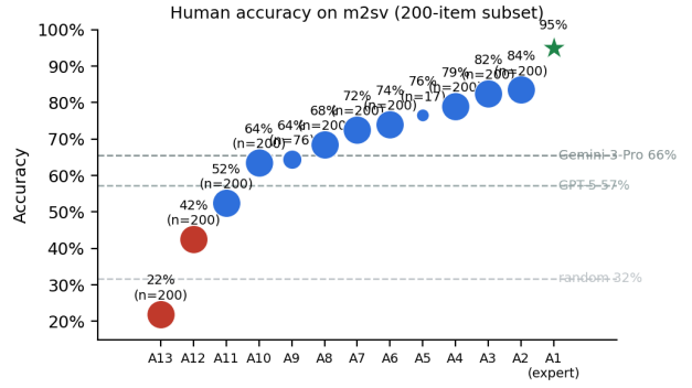
Figure 2. Per-annotator human accuracy on the 200-example subset (dot size \propto number of items answered). Annotators span 22%–84%; the two low-agreement outliers ( \kappa < 0.3 with the expert) are shown in red and the expert as a star. Dashed lines denote model and random baselines.
