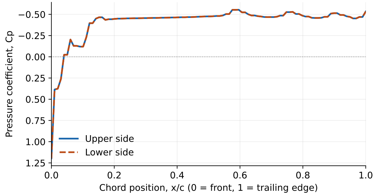
Near-surface Cp · negative values plotted upward
