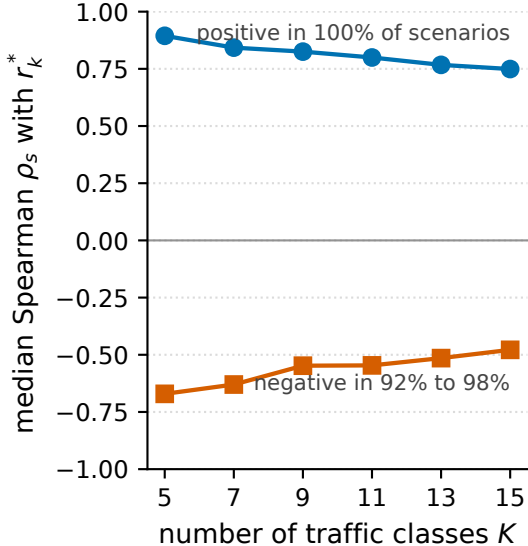
(b) effect size versus class count
