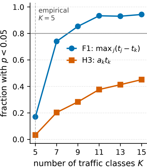
(a) power versus class count
