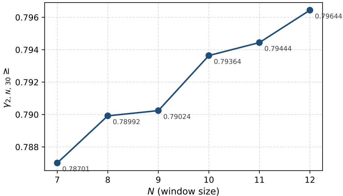
Lower bound on \gamma_2 versus window size N (MAX_SH=30)
