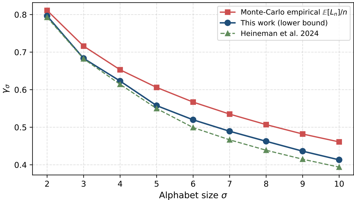
Lower bounds and Monte-Carlo for \gamma_\sigma , \sigma = 2, \dots, 10
