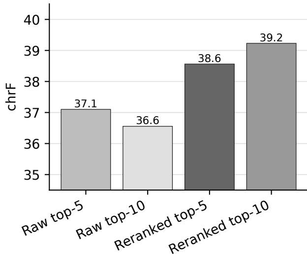
chrF
