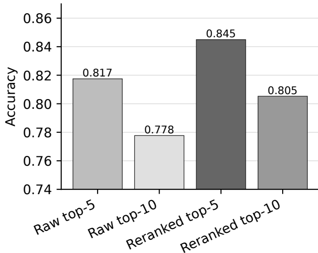
M-Prometheus accuracy
