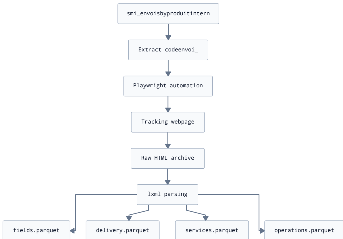
Figure A.1 - Tracking data acquisition pipeline
