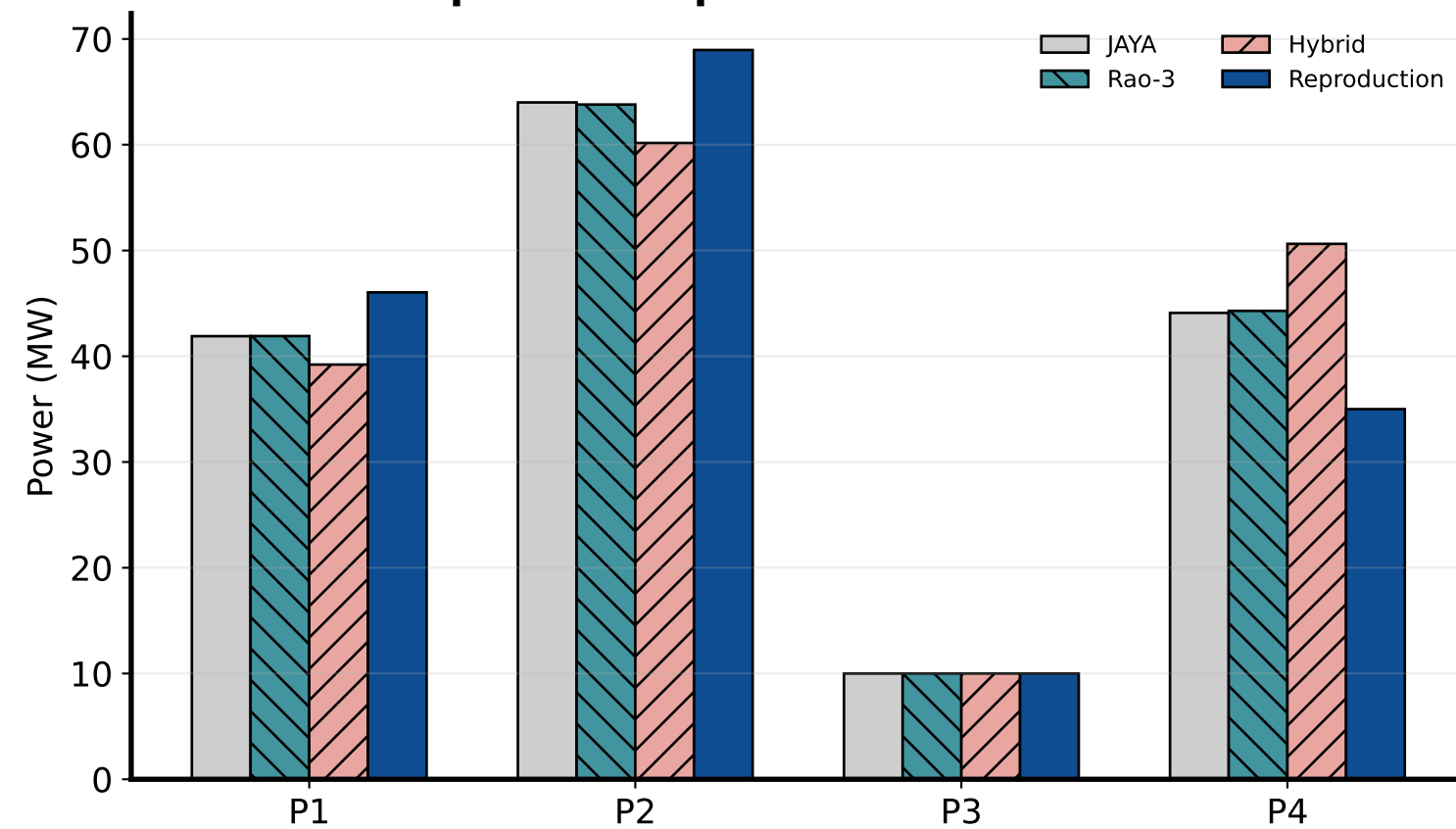
B. Electric Dispatch Comparison
