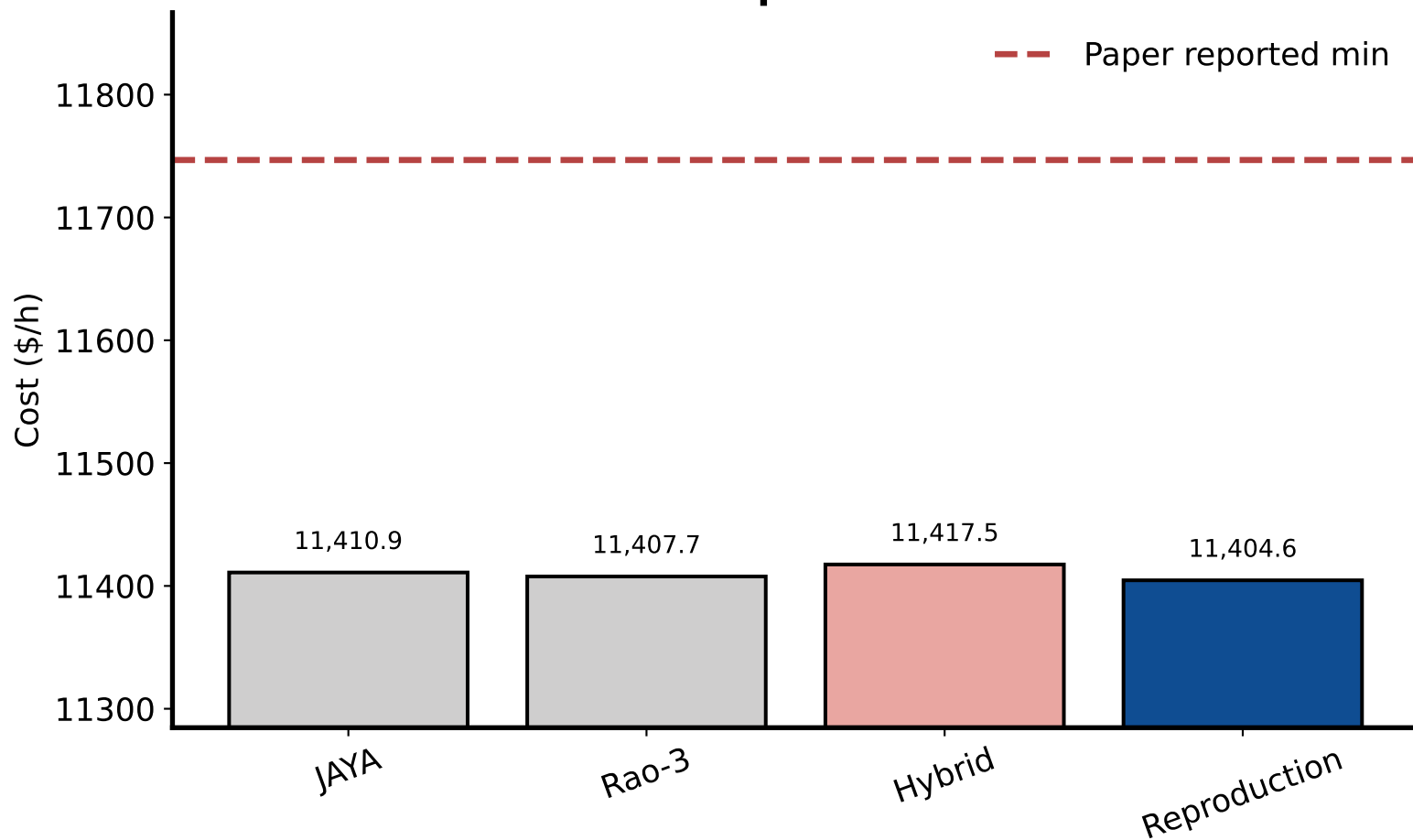
C. Heat Dispatch Comparison
