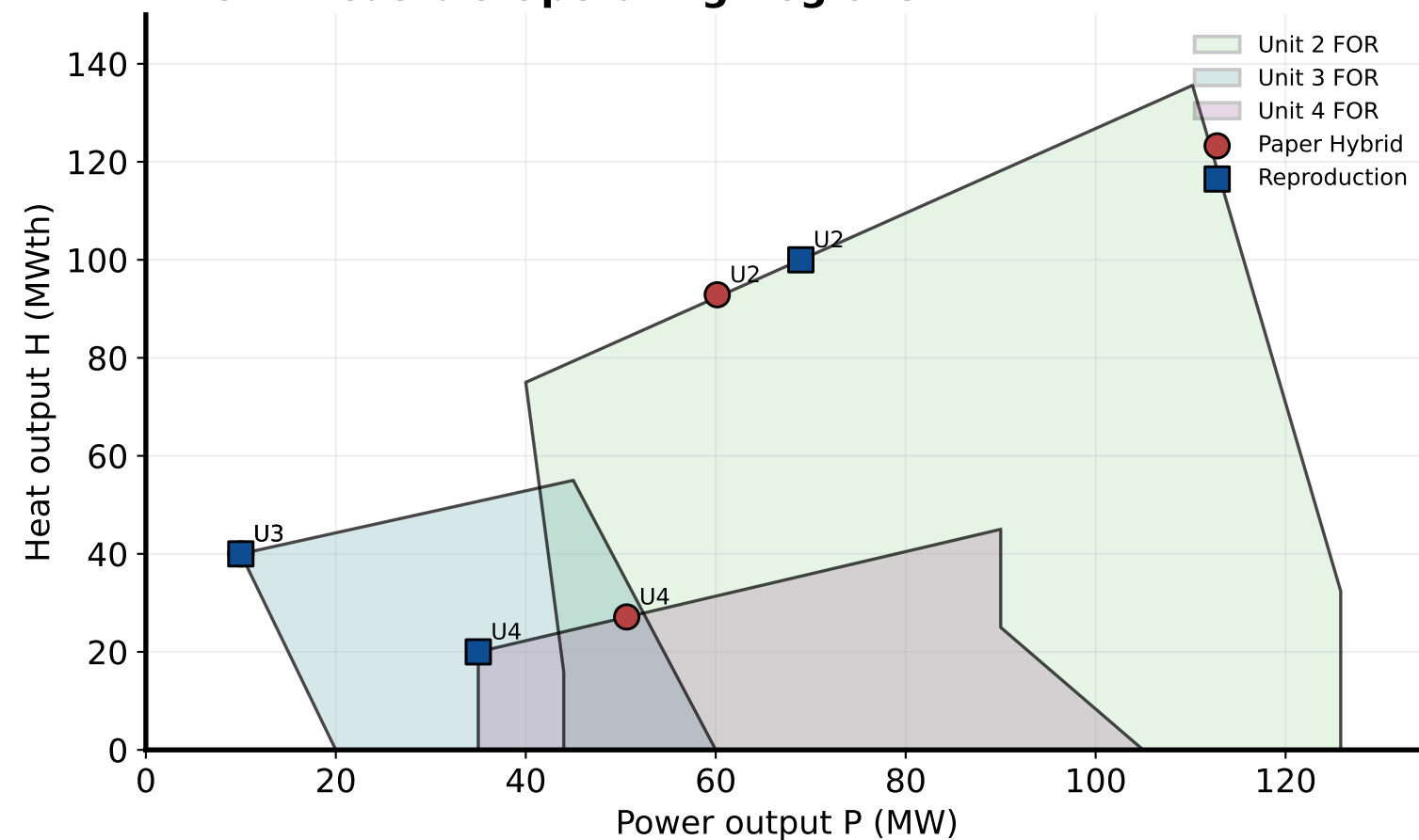
D. CHP Feasible Operating Regions
