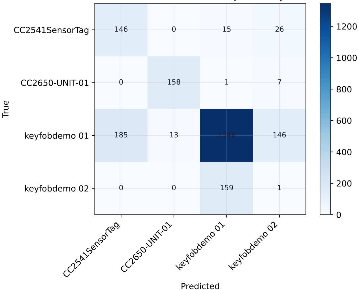
RQ1 -- confusion matrix (capture-disjoint)
