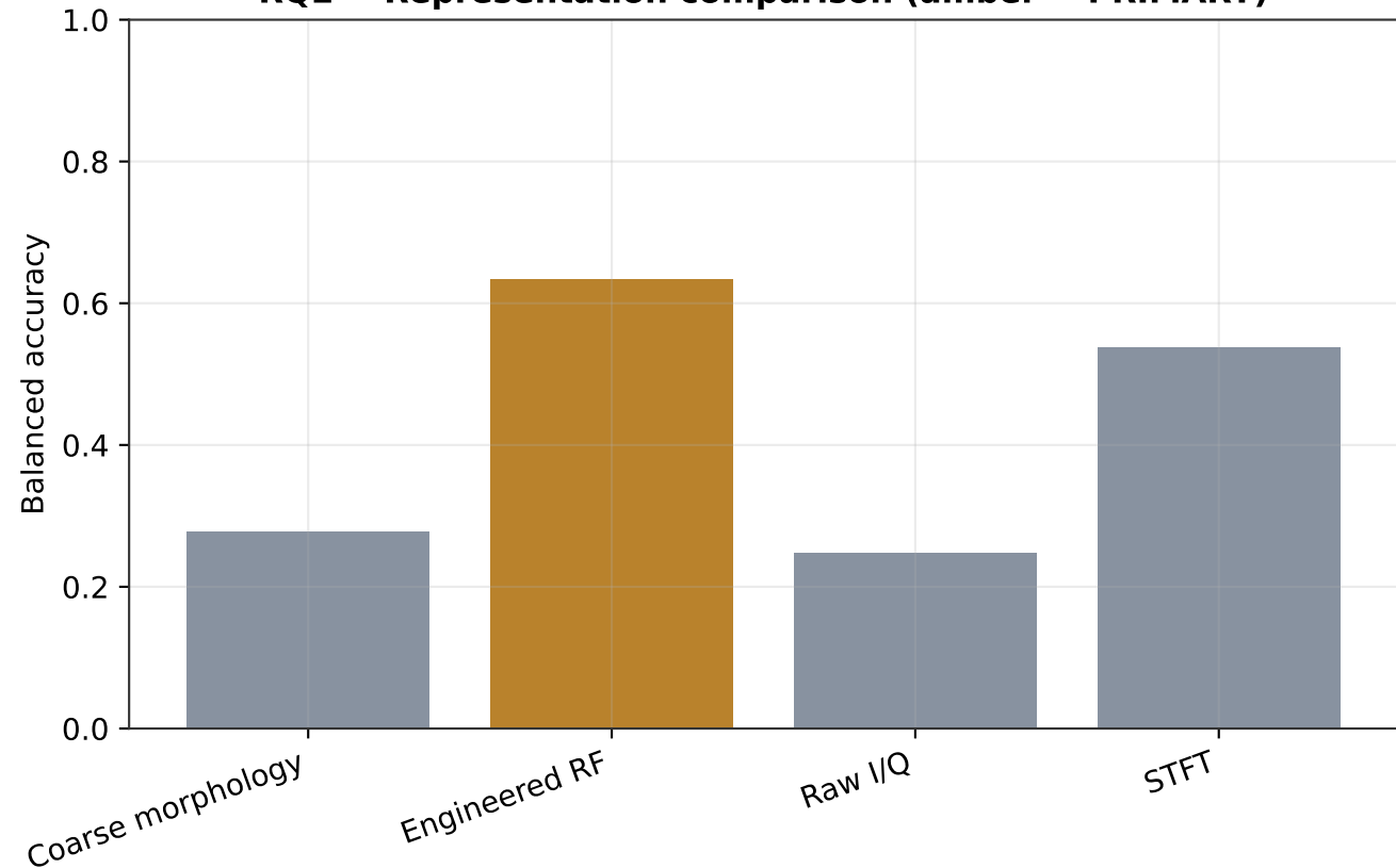
RQ2 -- Representation comparison (amber = PRIMARY)
