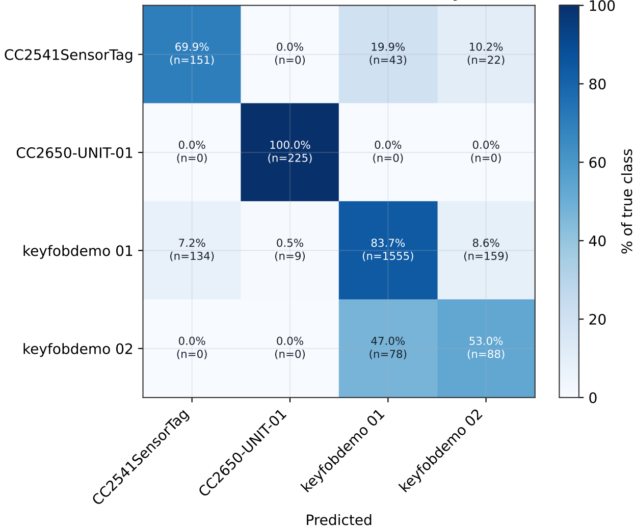
Closed-set -- confusion matrix, normalized by true class (TEST)
