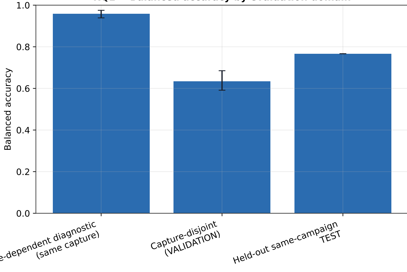
RQ1 -- Balanced accuracy by evaluation domain
