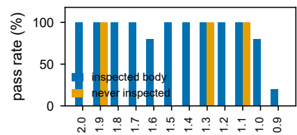
self-inspection and outcome, within each aperture
