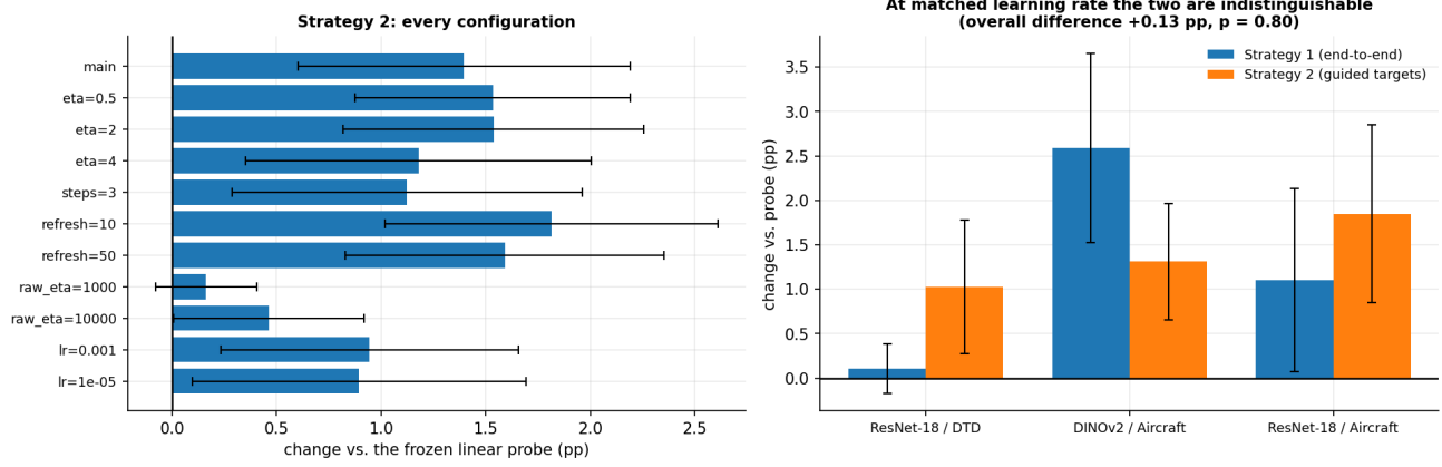
Figure 3. Every Strategy 2 configuration's \Delta against the frozen probe (left), and the strategy comparison at matched learning rate (right; see Section 7).
