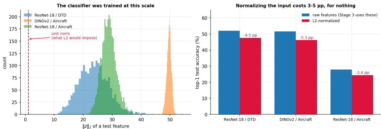
Figure 1. Feature-norm distributions per combination (left; the red line is the unit norm L2 normalisation would impose), and the measured accuracy cost of feeding the frozen classifier L2-normalised features instead of raw ones (right).
