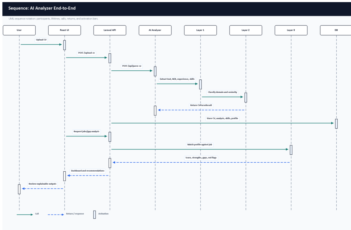
Figure 28. AI analyzer sequence diagram.
