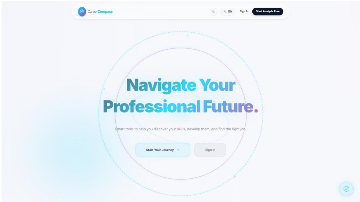
Figure 29. Home page.
