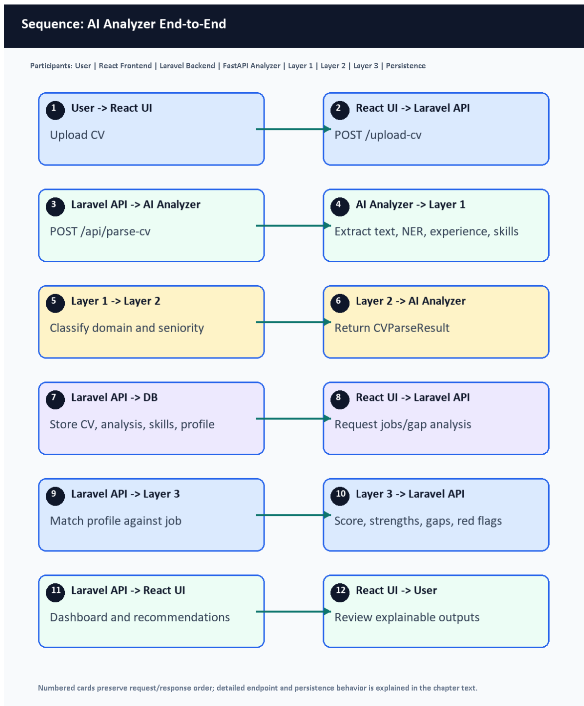
Figure 28. AI analyzer sequence diagram.
