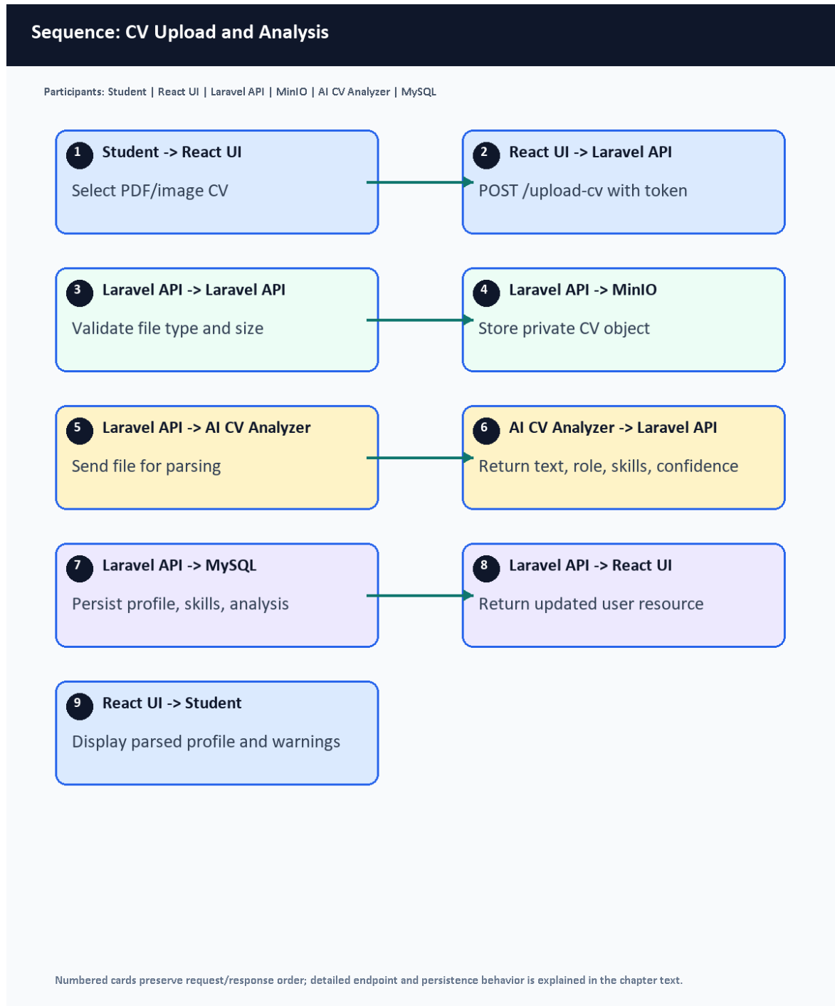
Figure 6. Sequence diagram for CV upload and analysis.
