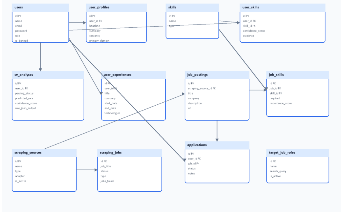
Figure 8. ERD and database summary diagram.
