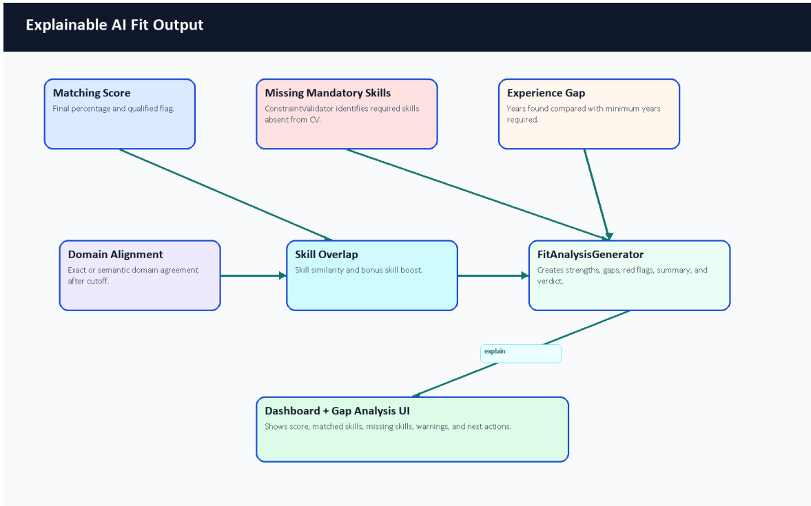
Figure 27. Explainable AI fit output.
