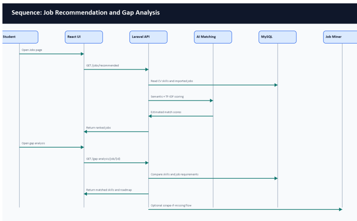
Image: Sequence diagram for recommendation and gap analysis.
