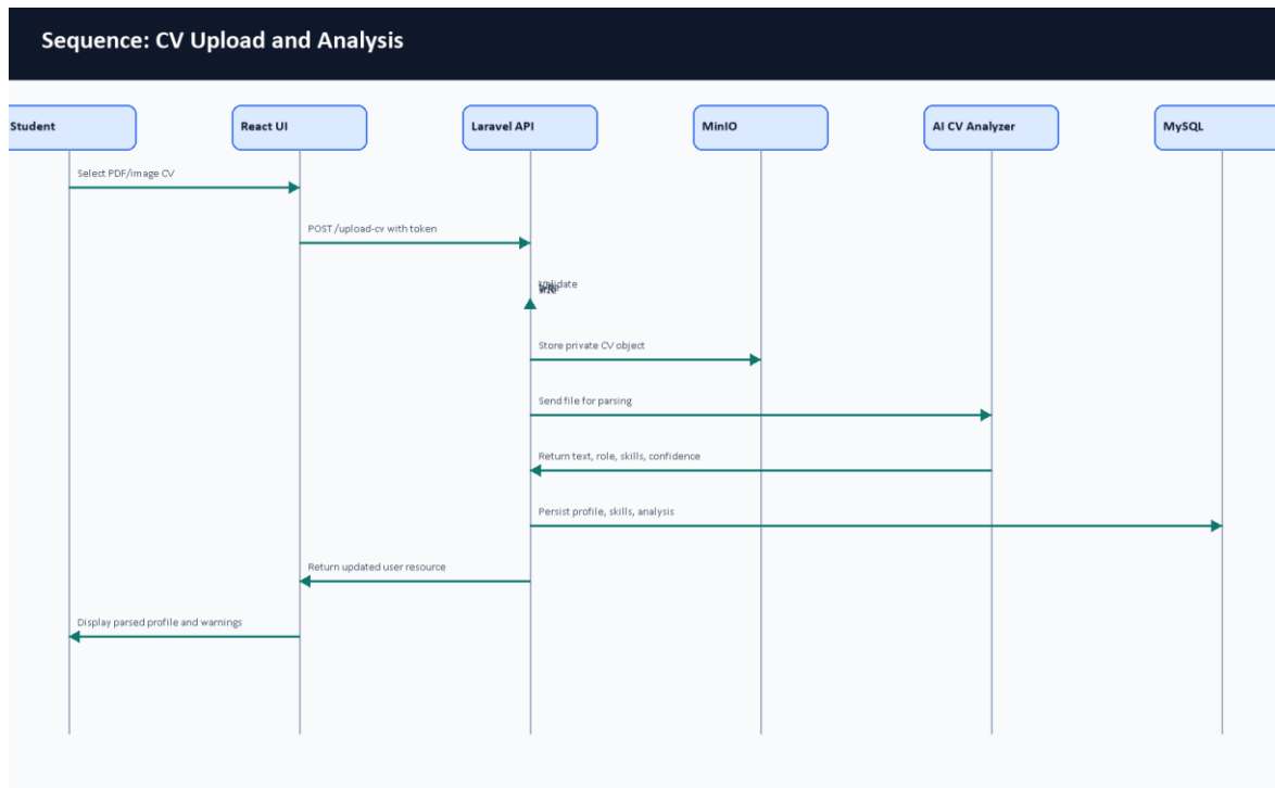
Image: Sequence diagram for CV upload and analysis.
