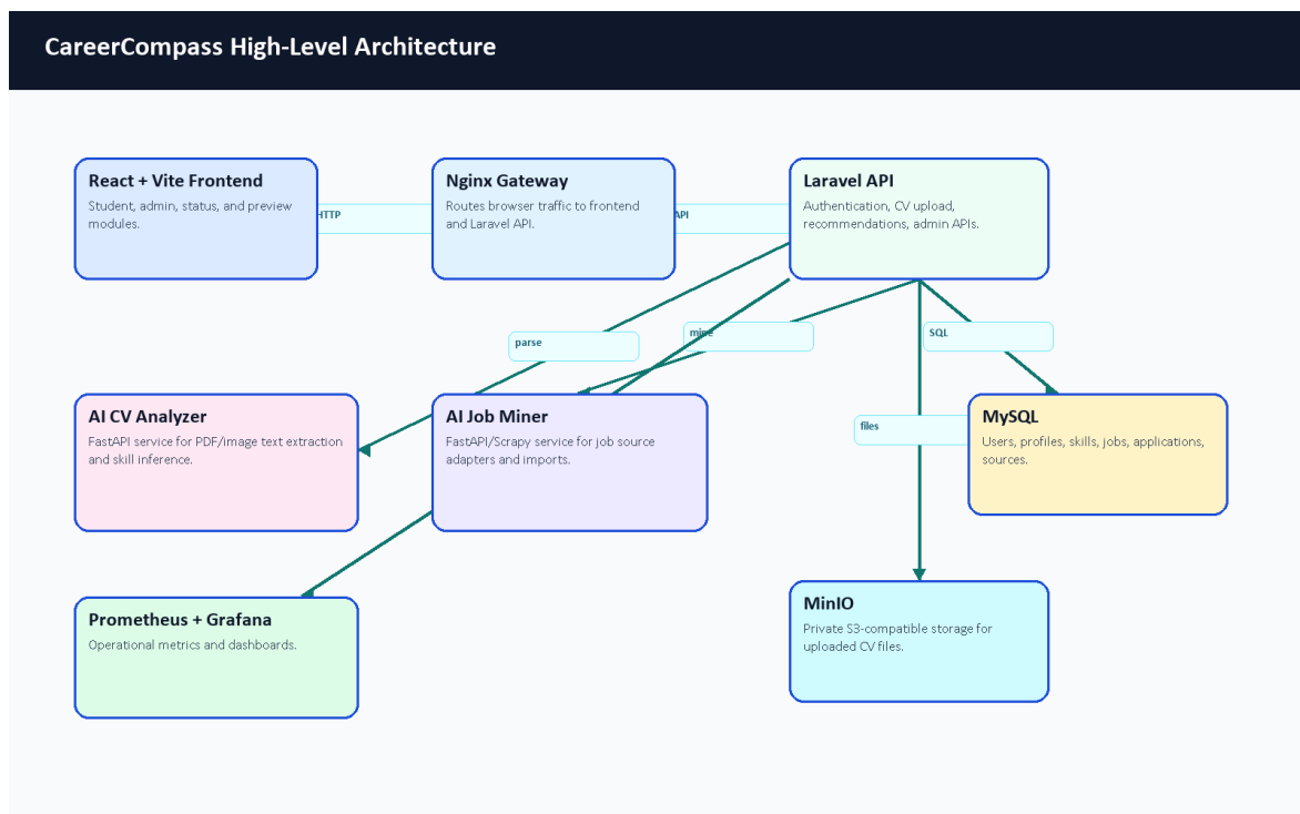
Image: High-level architecture of CareerCompass.
