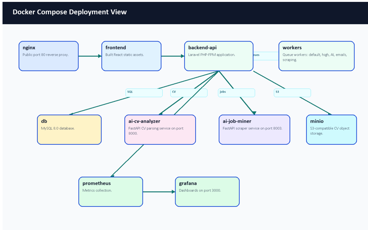
Image: Docker deployment architecture.
