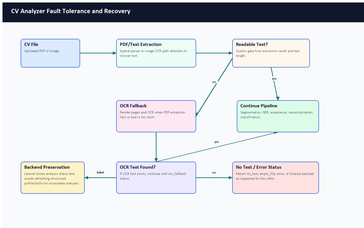
Figure 6.3. CV analyzer fault tolerance and recovery flow.
