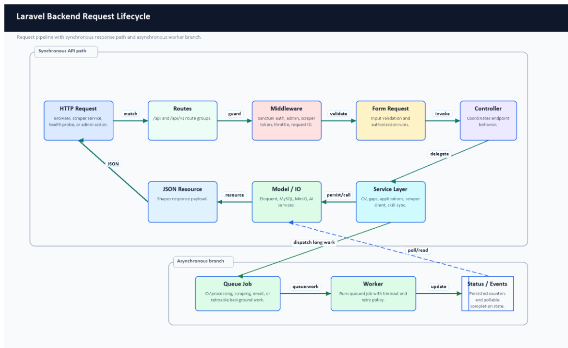
Figure 3.4. Laravel backend request lifecycle.
