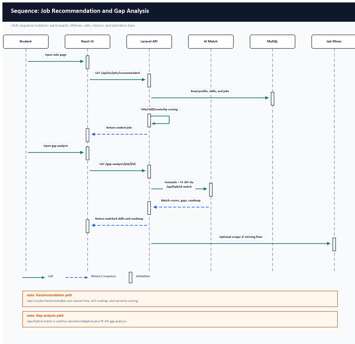
Figure 3.11. Sequence diagram for recommendation and gap analysis.
