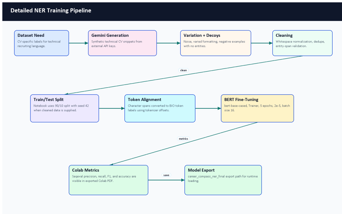
Figure 6.7. Detailed NER training pipeline.
