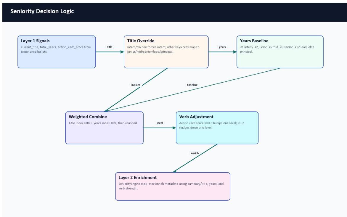
Figure 5.9. Seniority decision logic.
