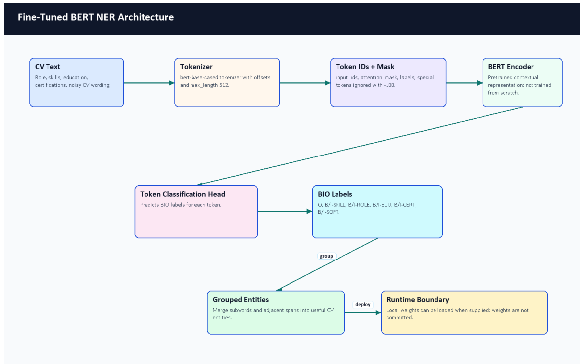
Figure 6.6. Fine-tuned BERT NER architecture.
