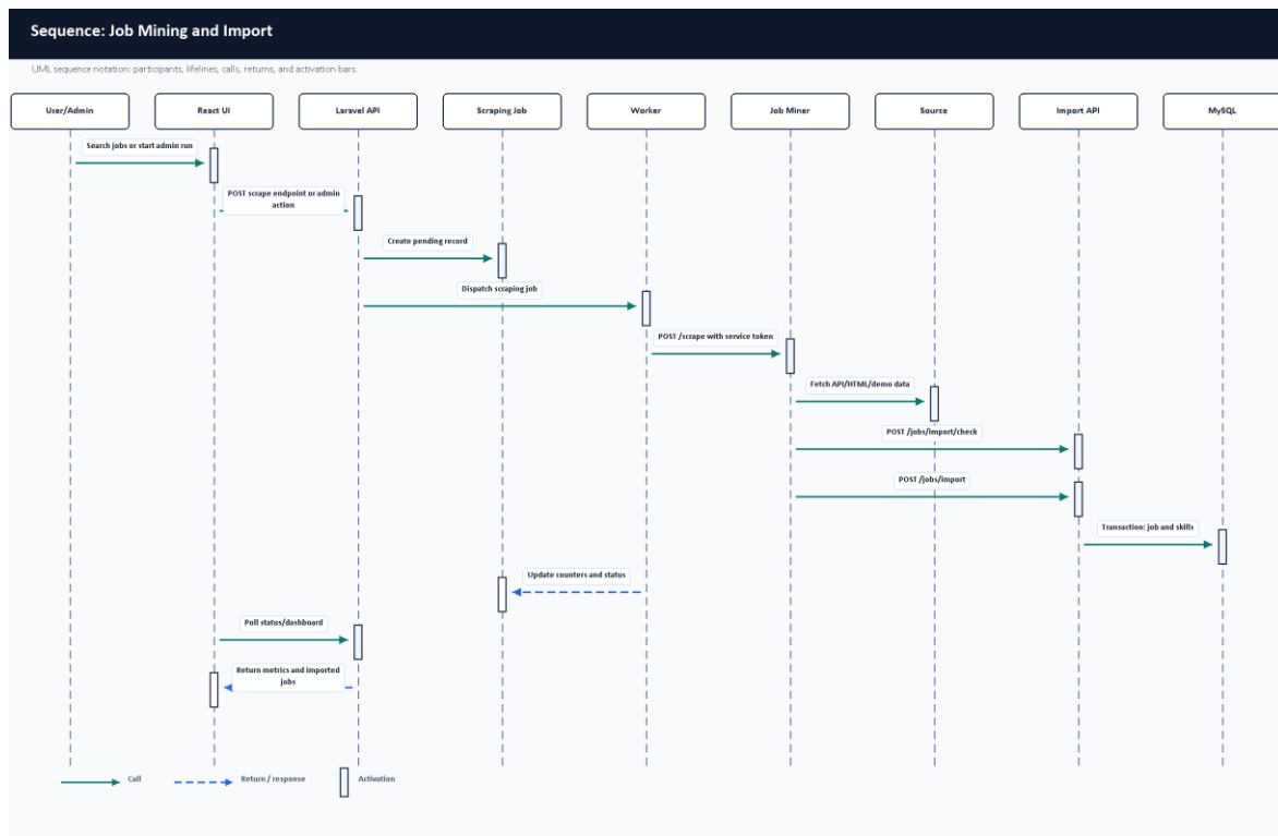
Figure 7.4. Scraping sequence diagram.
