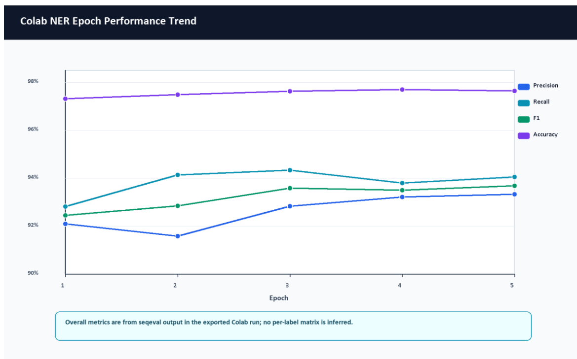
Figure 6.10. Colab NER epoch performance trend.
