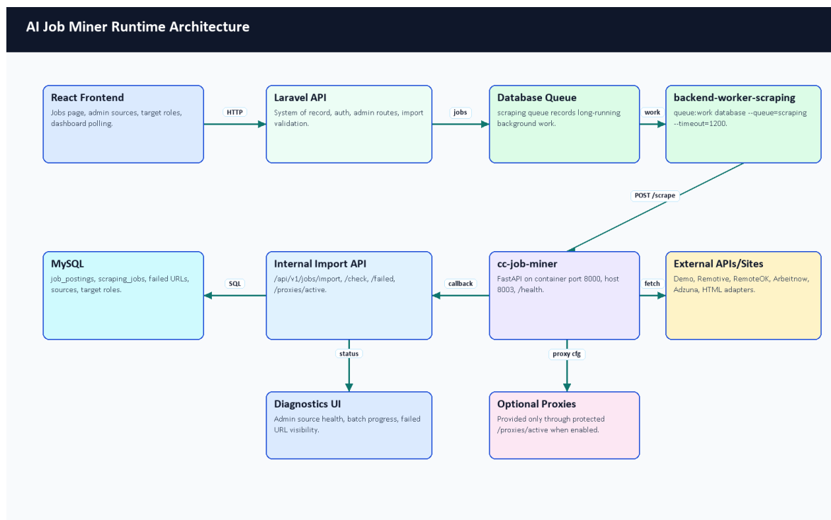
Figure 7.2. AI Job Miner runtime architecture.
