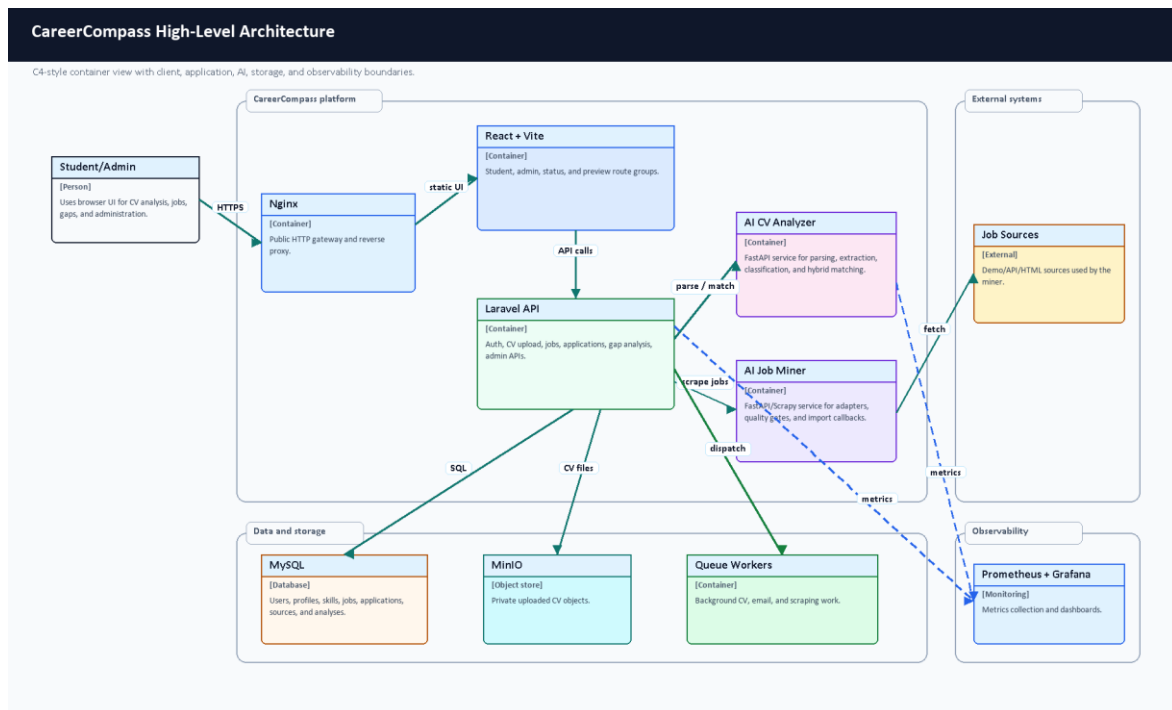
Figure 3.1. High-level architecture of CareerCompass.
