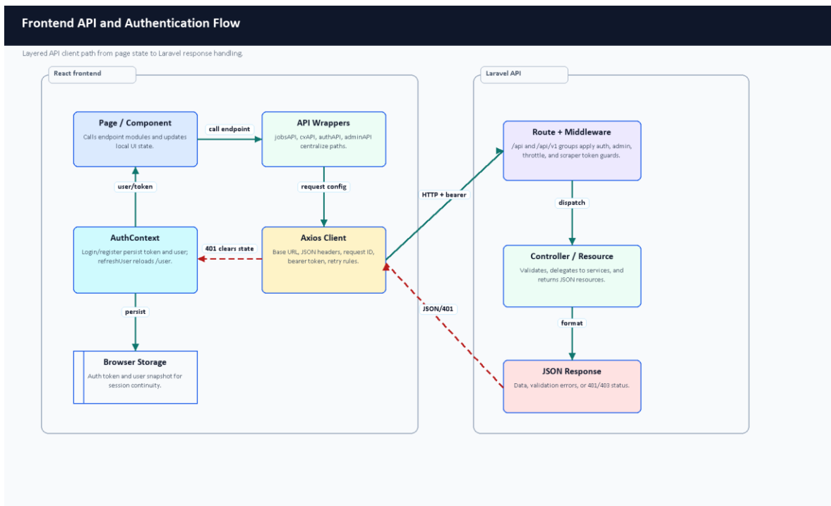
Figure 3.3. Frontend API and authentication flow.
