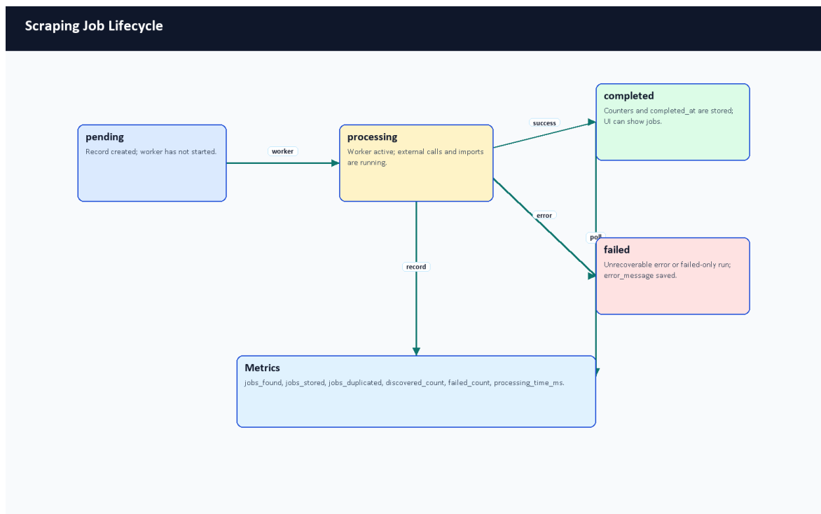
Figure 7.5. Scraping job lifecycle.
