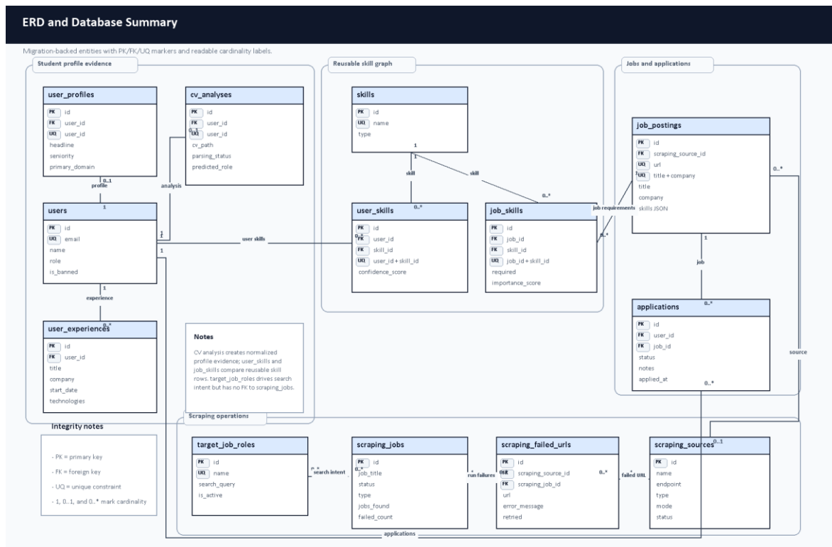
Figure 3.7. ERD and database summary diagram.
