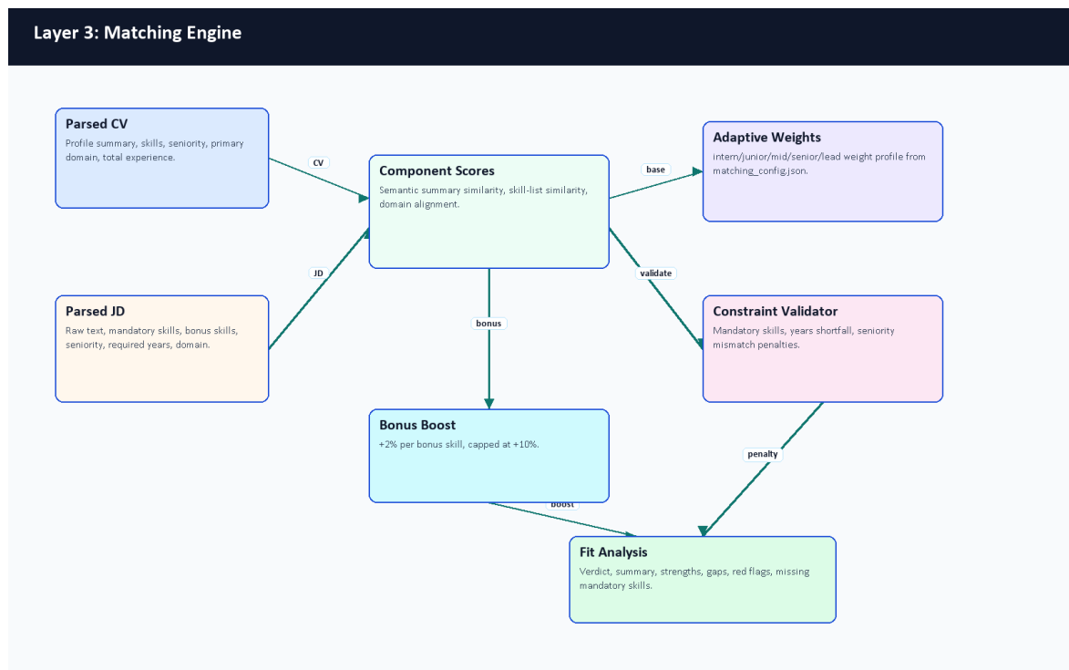
Figure 5.10. Layer 3 matching engine.
