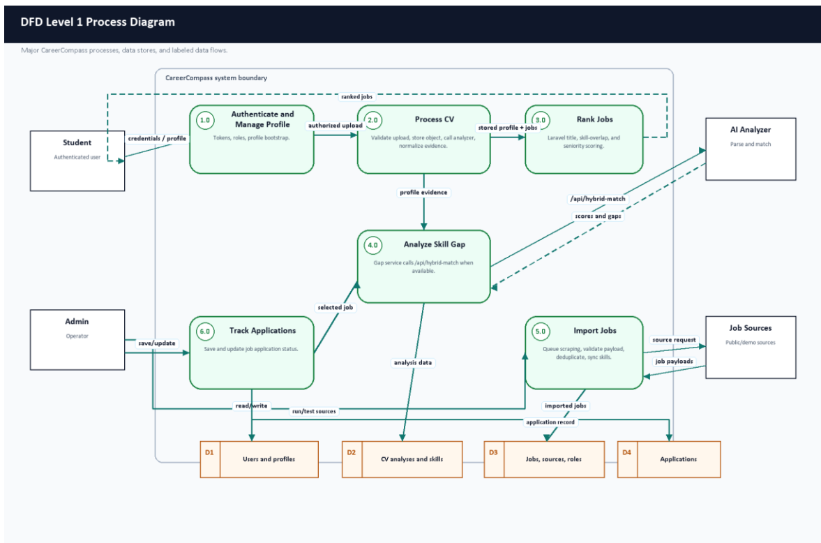
Figure 3.9. DFD Level 1 process diagram.
