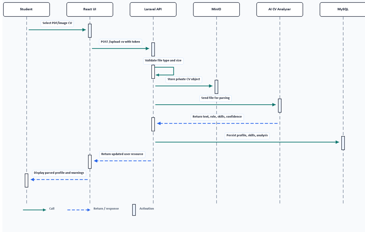
Figure 3.10. Sequence diagram for CV upload and analysis.
