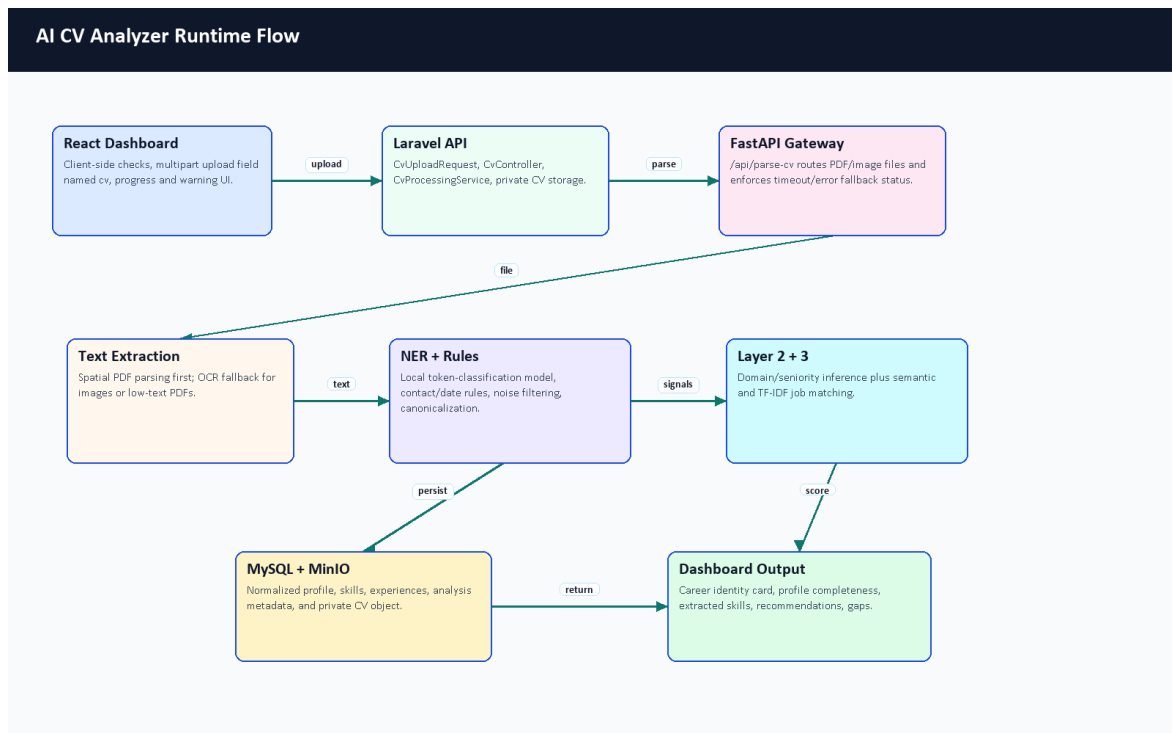
Figure 3.5. AI CV Analyzer runtime flow.
