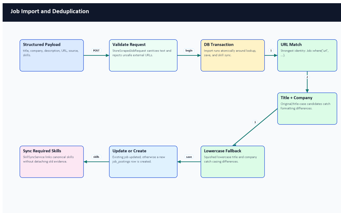
Figure 7.7. Job import and deduplication flow.
