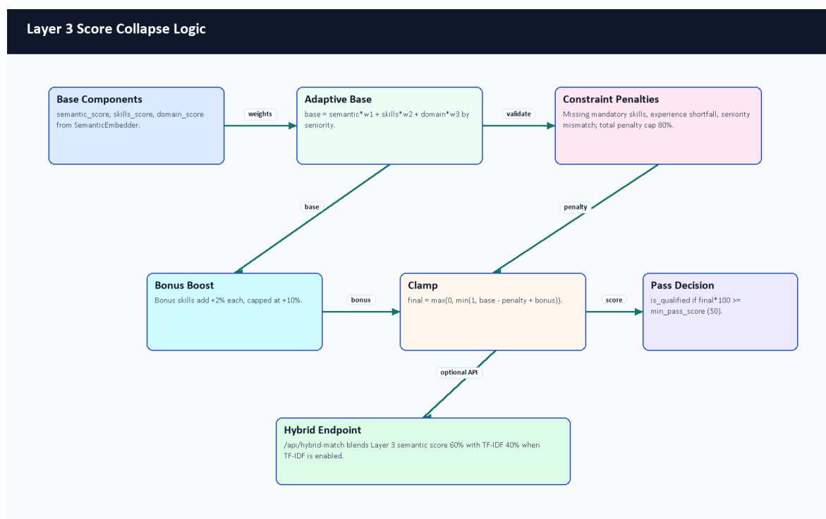
Figure 5.11. Layer 3 score collapse logic.
