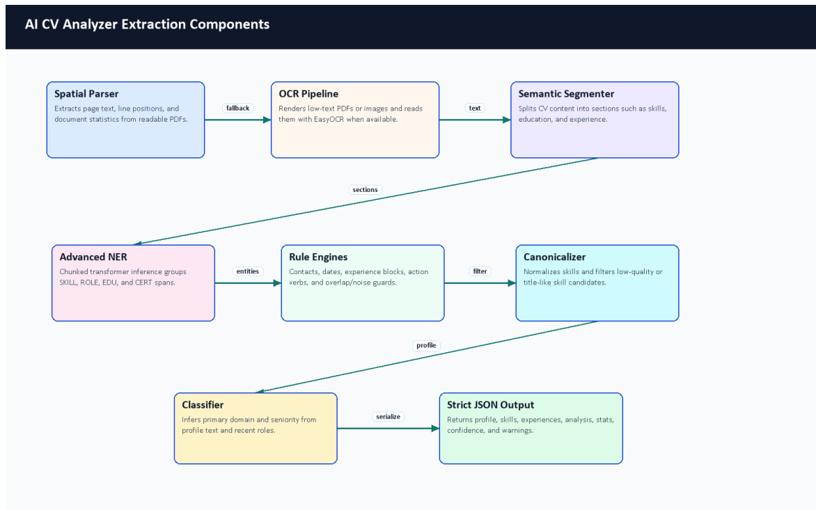
Figure 5.4. AI CV Analyzer extraction components.
