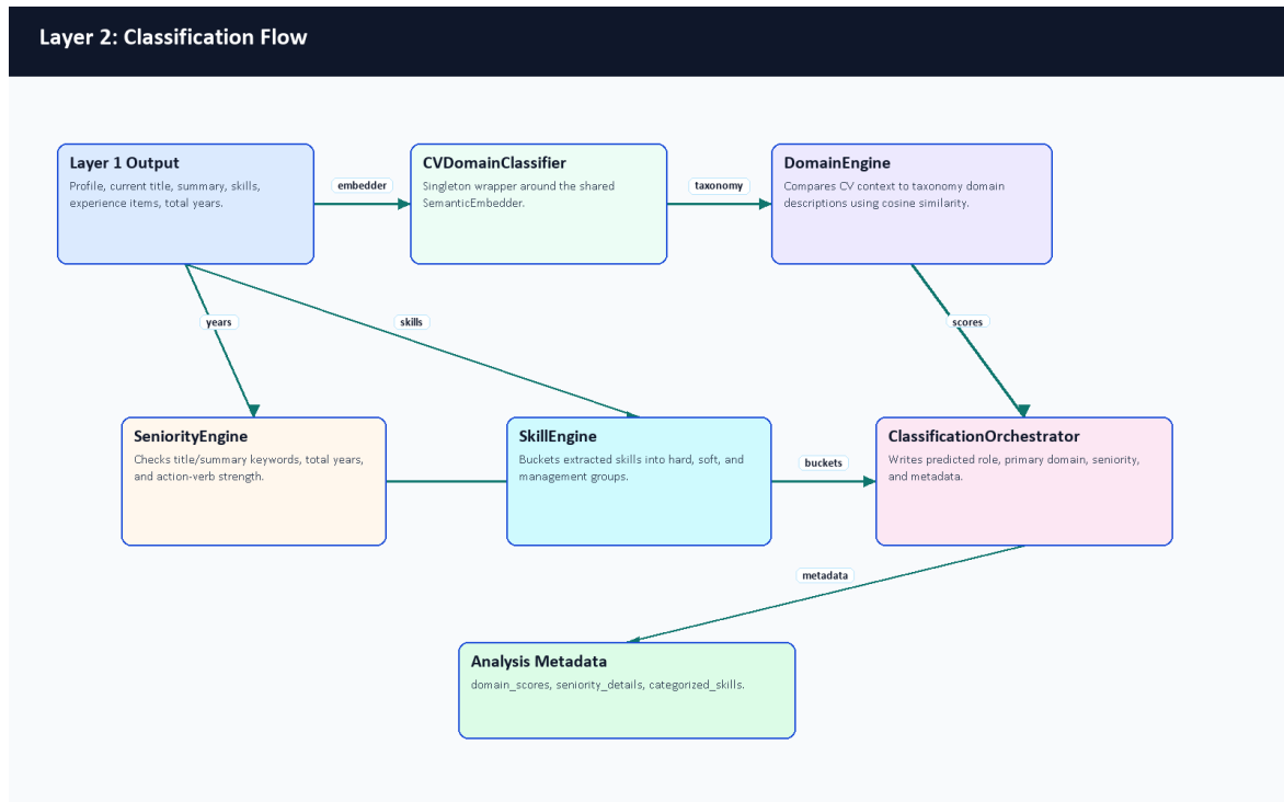
Figure 5.8. Layer 2 classification flow.
