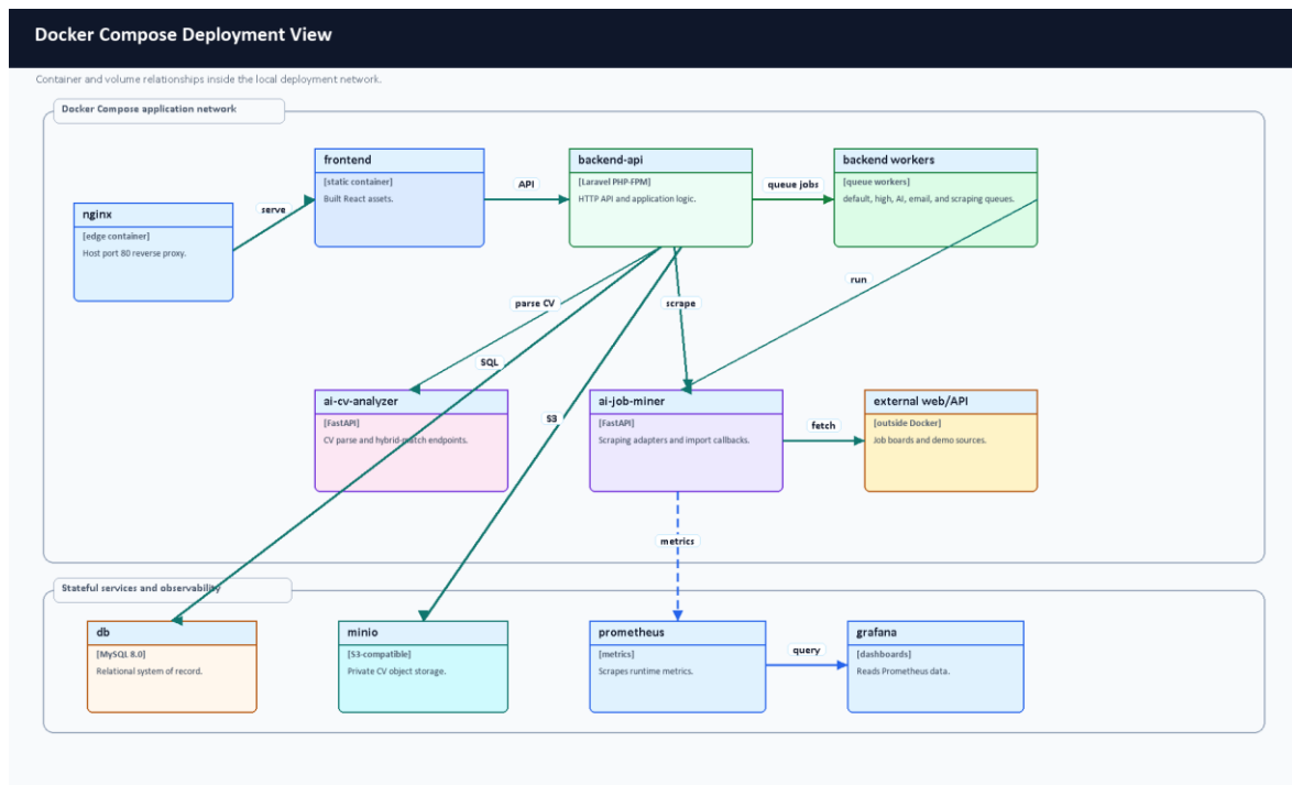
Figure 3.12. Docker deployment architecture.
