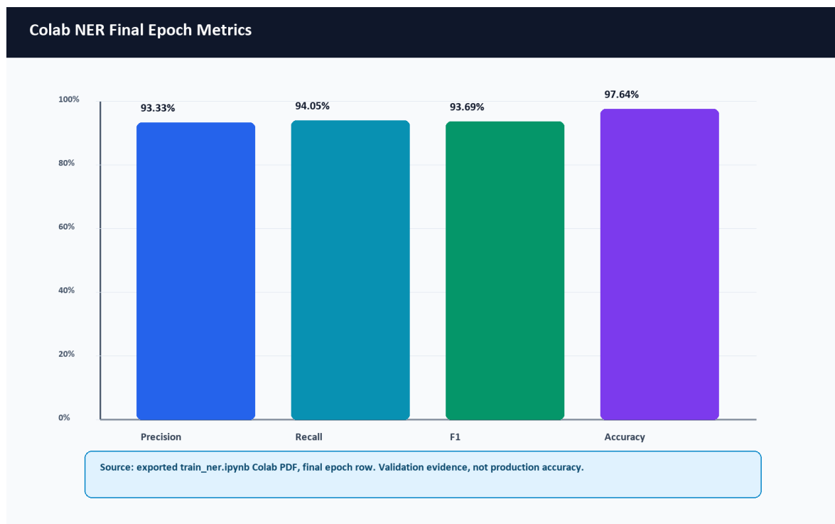
Figure 6.9. Colab NER final epoch metrics.
