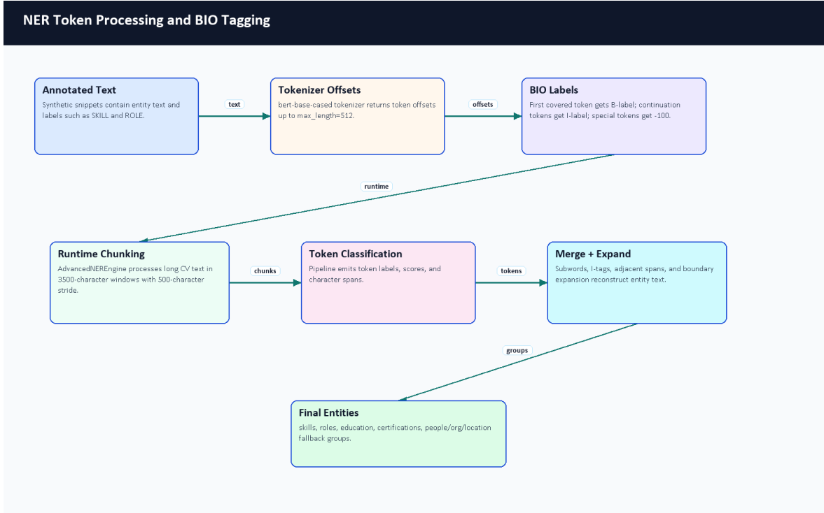
Figure 15. NER token processing and BIO tagging.
