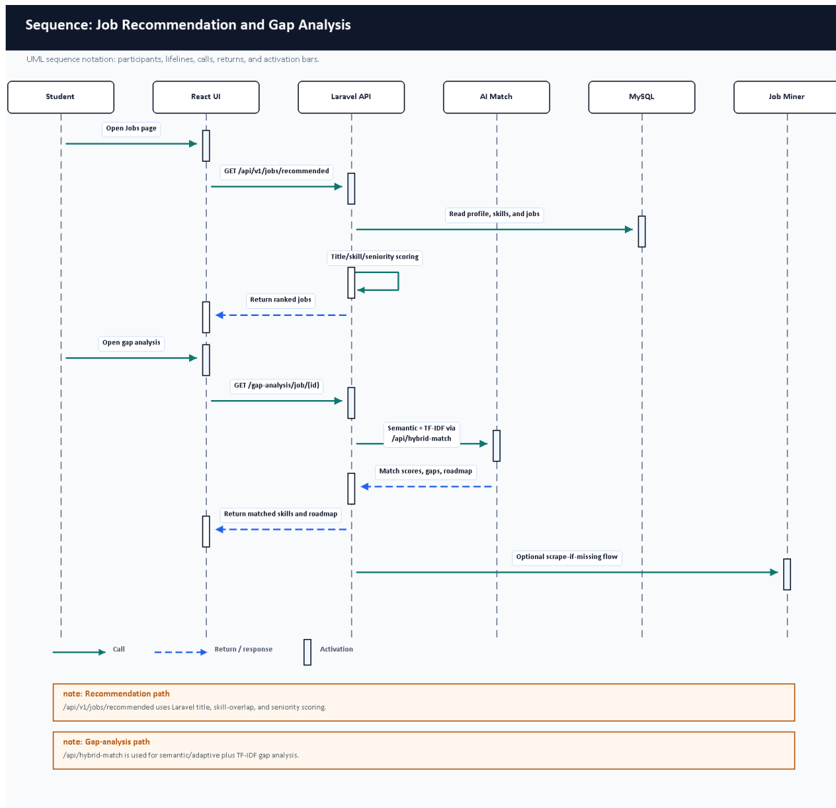
Figure 7. Sequence diagram for recommendation and gap analysis.
