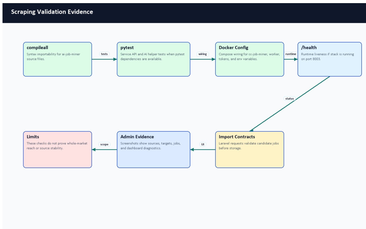
Figure 62. Scraping validation evidence.
