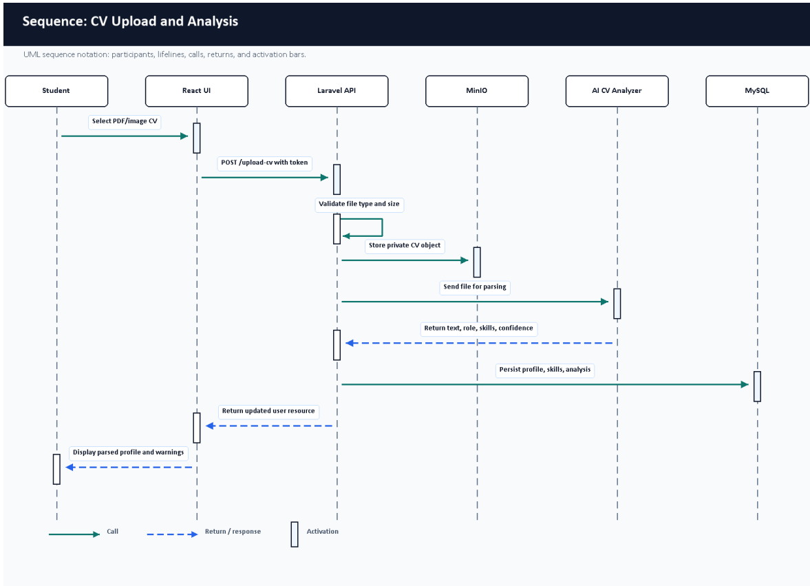
Figure 6. Sequence diagram for CV upload and analysis.
