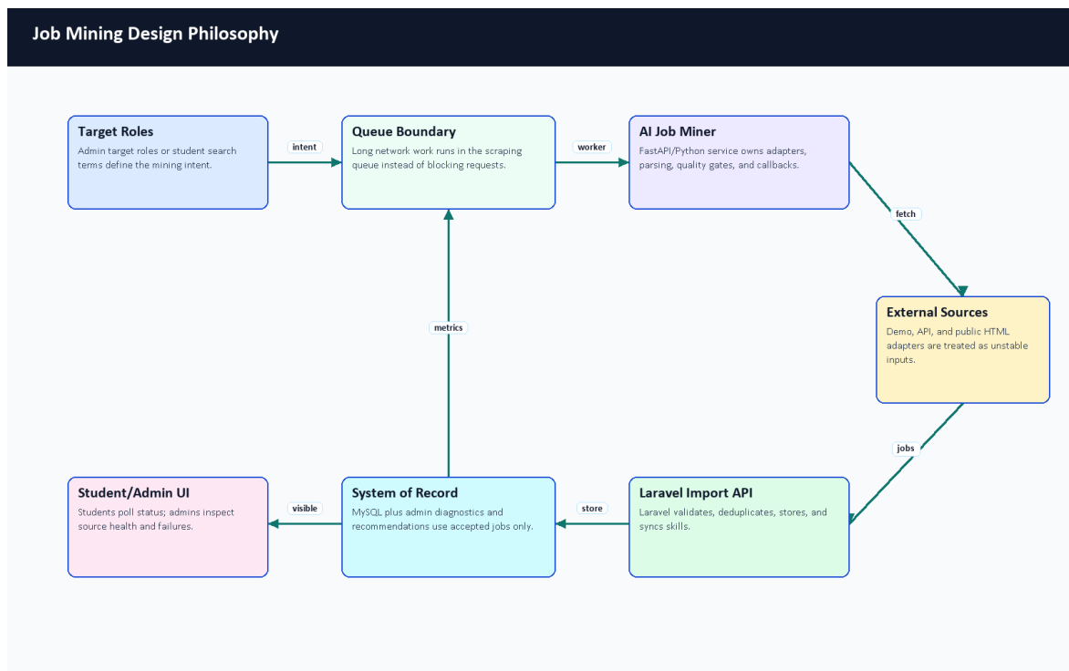
Figure 53. Job mining design philosophy.
