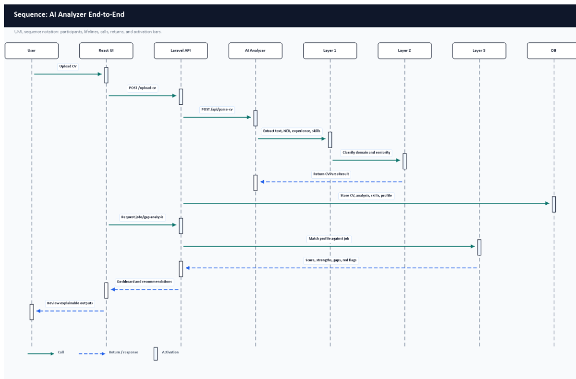
Figure 28. AI analyzer sequence diagram.
