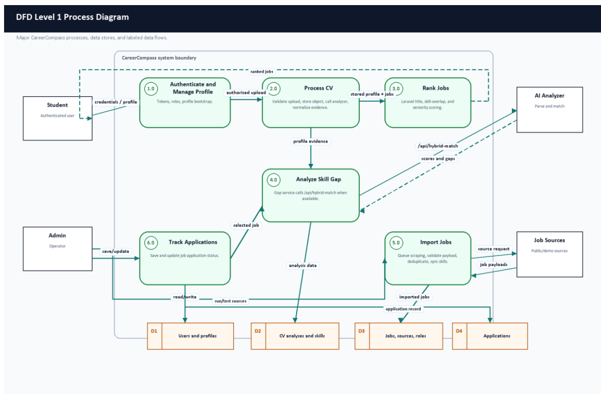
Figure 4. DFD Level 1 process diagram.
