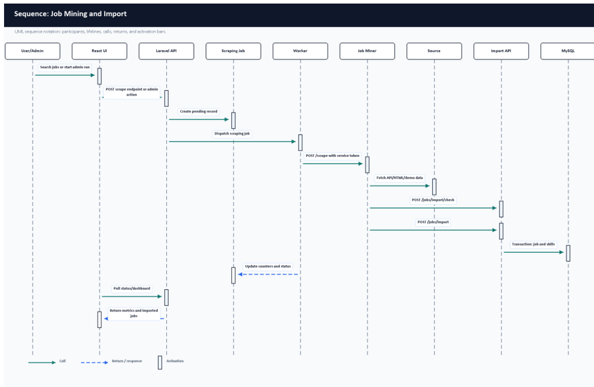
Figure 56. Scraping sequence diagram.
