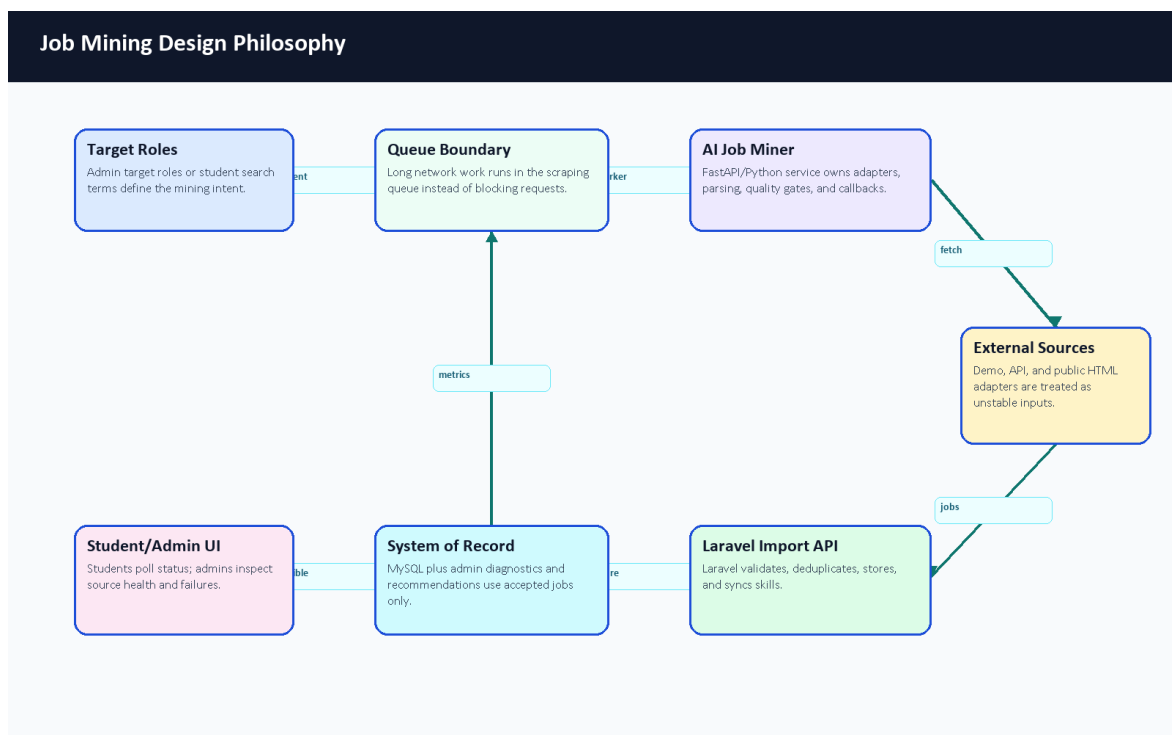
Figure 51. Job mining design philosophy.
