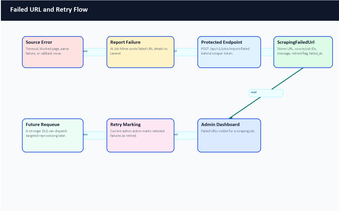
Figure 58. Failed URL and retry flow.
