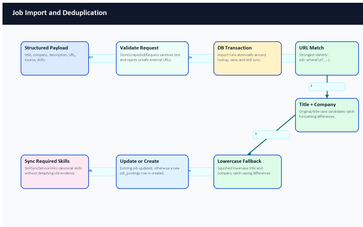
Figure 57. Job import and deduplication flow.
