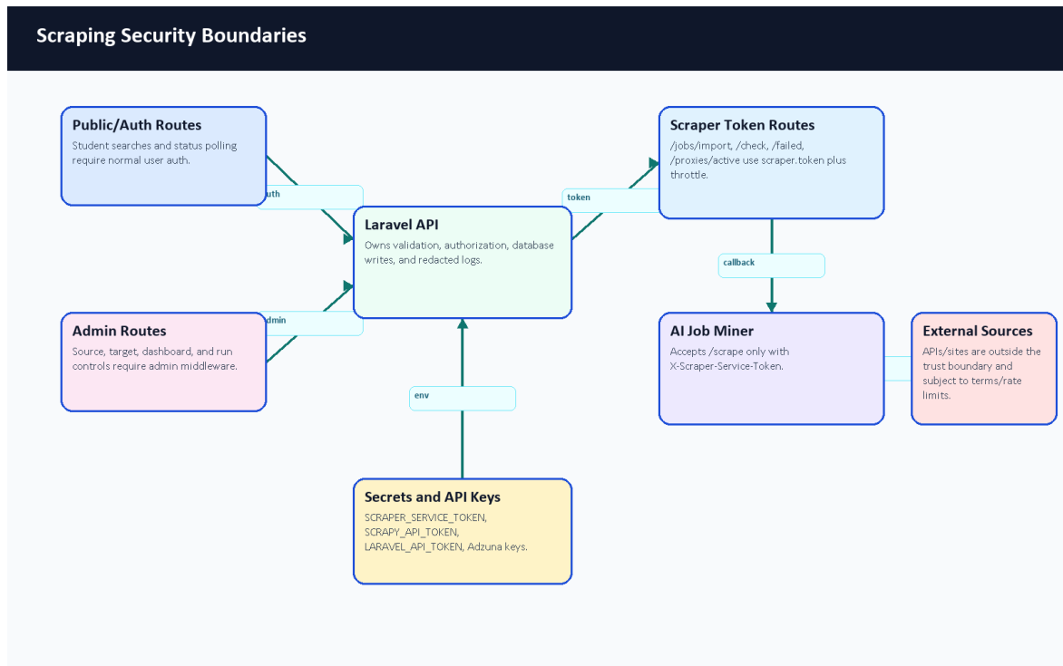
Figure 59. Scraping security boundaries.
