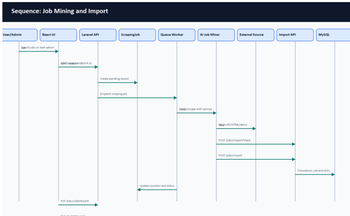
Figure 54. Scraping sequence diagram.
