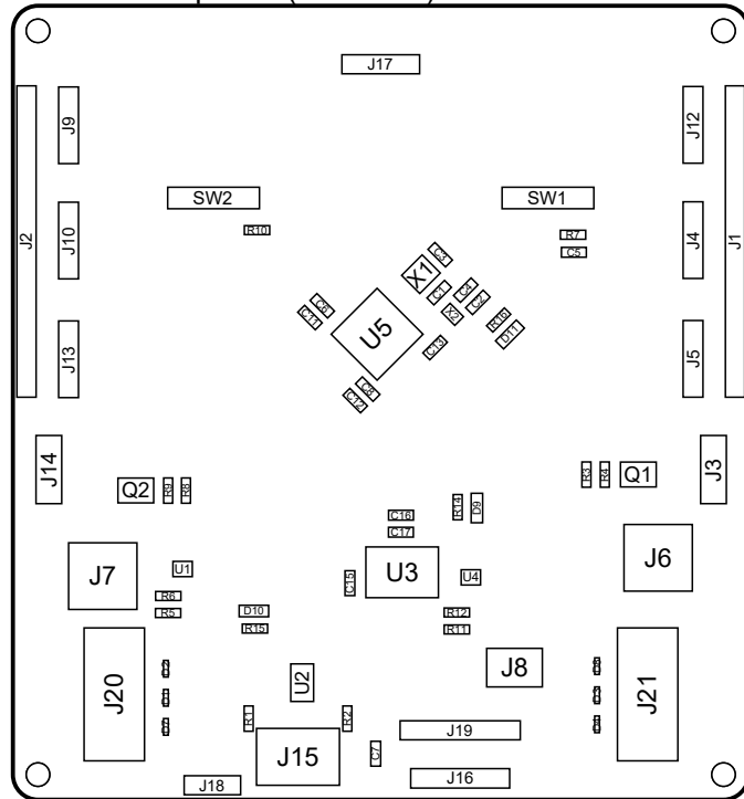
View from Front side (Scale 1:1)
