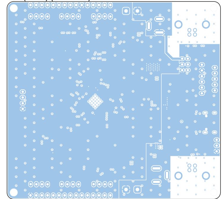
Int2 (PWR) (Scale 1:1)
