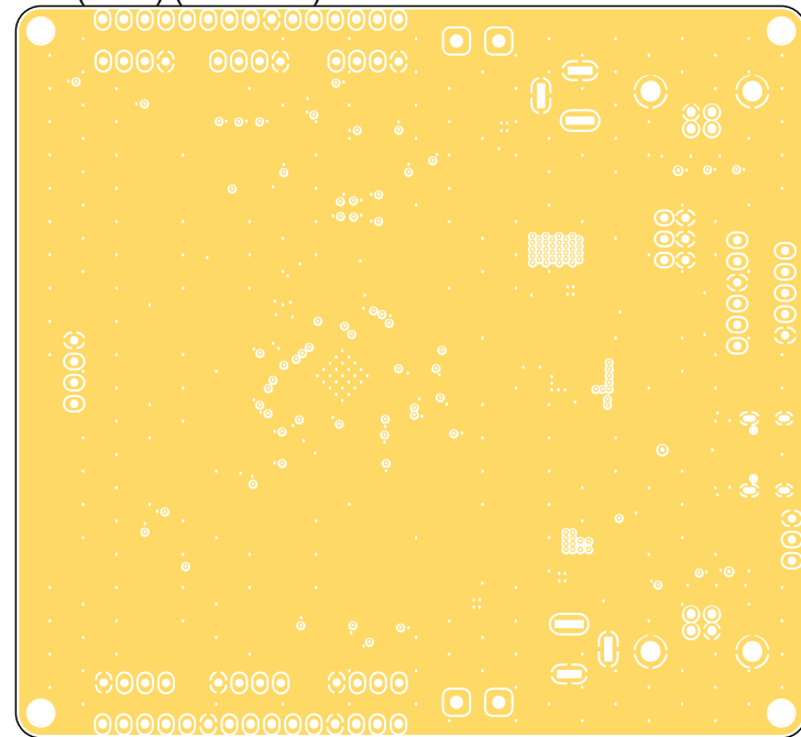
Int1 (GND) (Scale 1:1)
