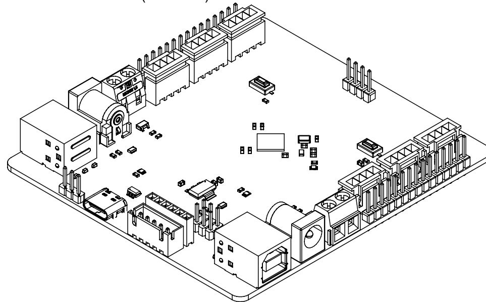
View from Front side (Scale 1:1)
