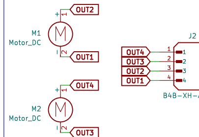
DC Motors N20
