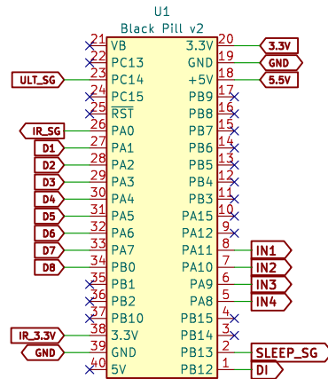
STM32 Black Pill
