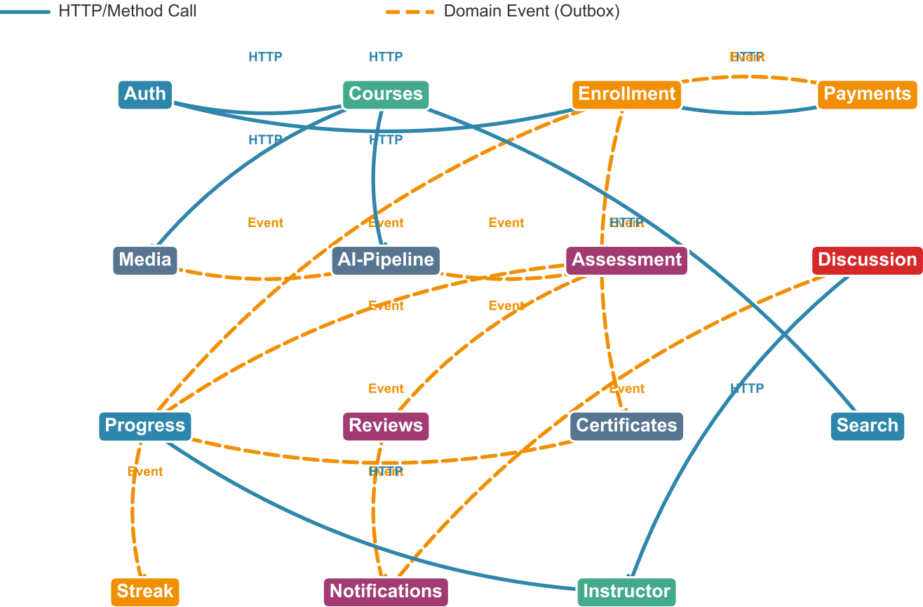
Figure 4.2 — Module Interaction Diagram (Bounded Context Dependencies)
